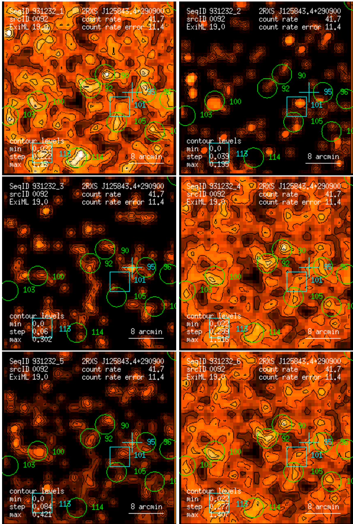
Figure 92: RASS 931232: detection 0092: band rate images, Gaussian filter: (1) PSPC channels 11 – 41, (2) 52 – 90, (3) 91 – 201, (4) 11 – 235, (5) 52 – 201, (6) 11 – 201. Broad band rates in counts/ks. Band rate contour levels in counts/ks/arcmin 2 .
