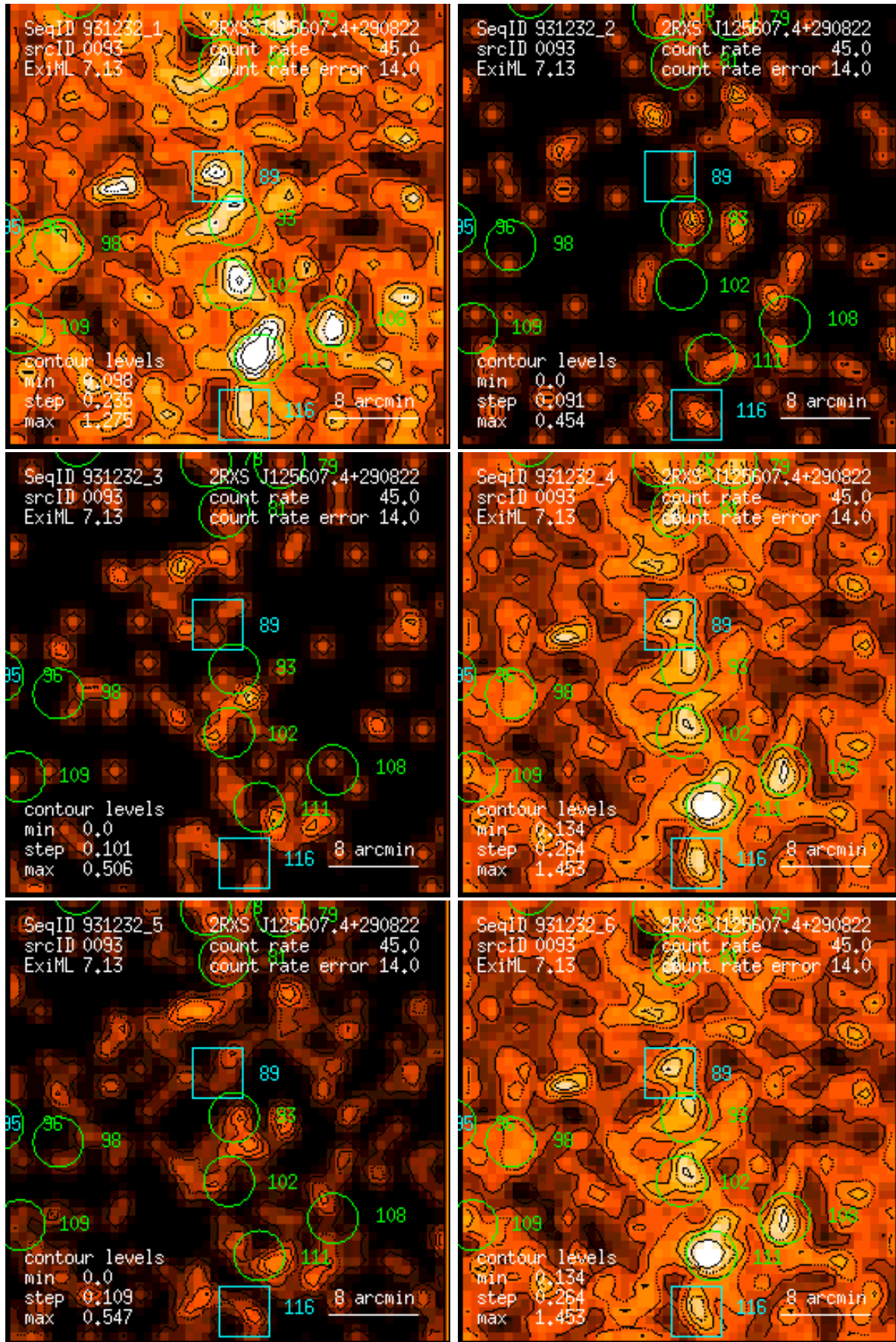
Figure 93: RASS 931232: detection 0093: band rate images, Gaussian filter: (1) PSPC channels 11 – 41, (2) 52 – 90, (3) 91 – 201, (4) 11 – 235, (5) 52 – 201, (6) 11 – 201. Broad band rates in counts/ks. Band rate contour levels in counts/ks/arcmin 2 .
