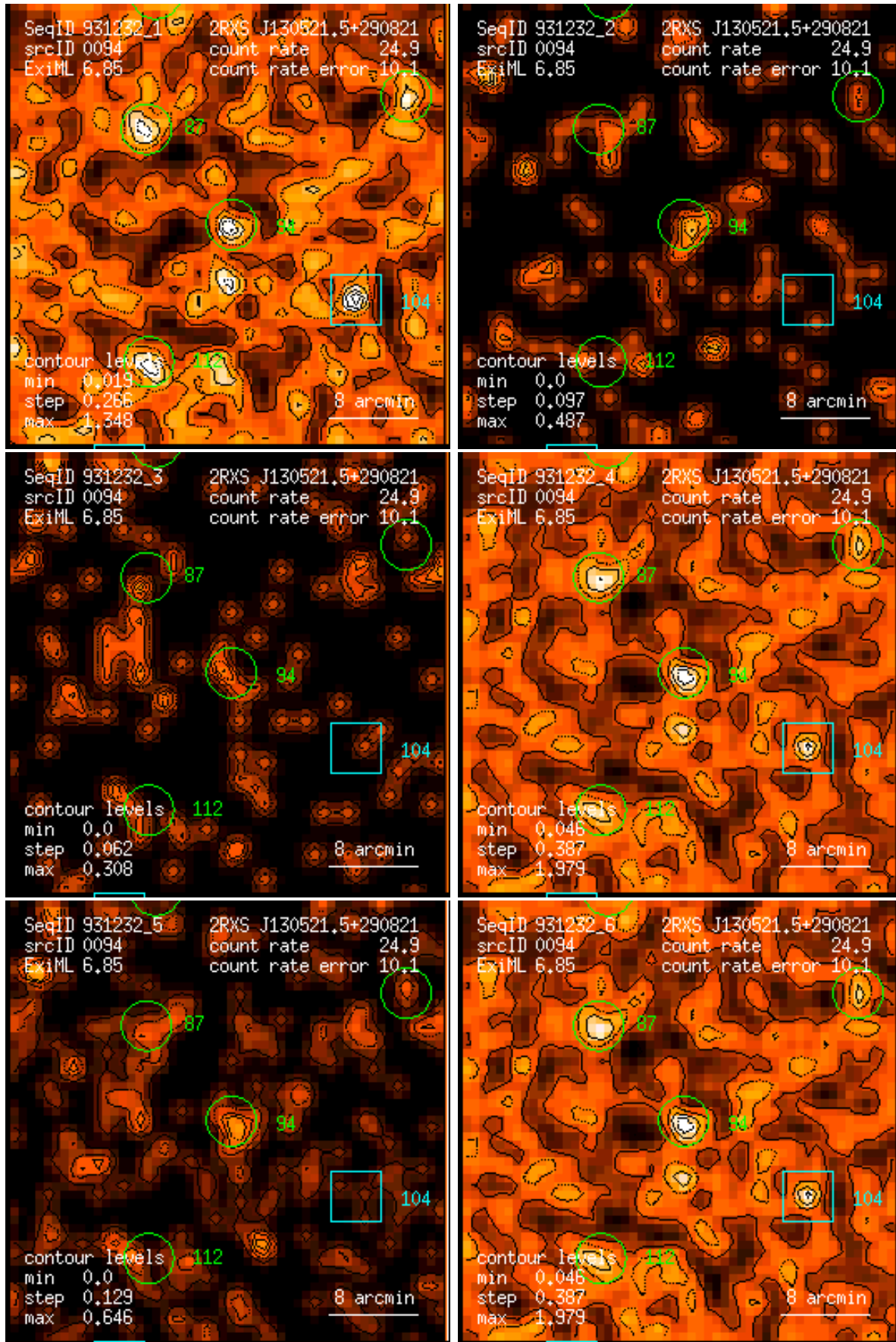
Figure 94: RASS 931232: detection 0094: band rate images, Gaussian filter: (1) PSPC channels 11 – 41, (2) 52 – 90, (3) 91 – 201, (4) 11 – 235, (5) 52 – 201, (6) 11 – 201. Broad band rates in counts/ks. Band rate contour levels in counts/ks/arcmin 2 .
