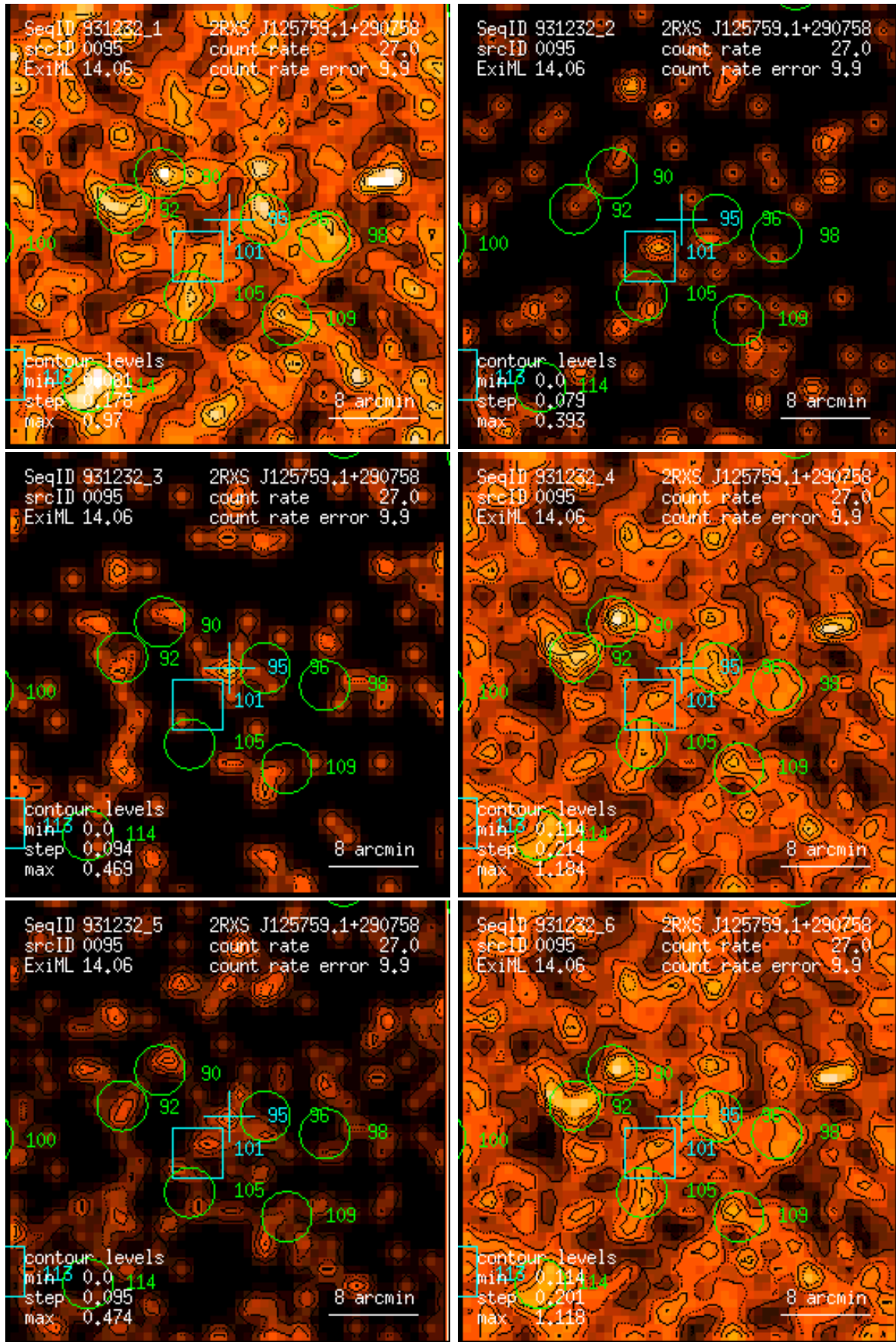
Figure 95: RASS 931232: detection 0095: band rate images, Gaussian filter: (1) PSPC channels 11 – 41, (2) 52 – 90, (3) 91 – 201, (4) 11 – 235, (5) 52 – 201, (6) 11 – 201. Broad band rates in counts/ks. Band rate contour levels in counts/ks/arcmin 2 .
