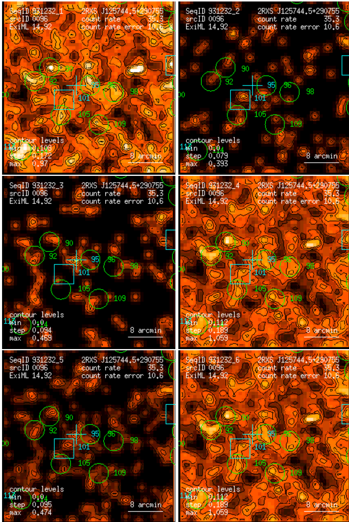
Figure 96: RASS 931232: detection 0096: band rate images, Gaussian filter: (1) PSPC channels 11 – 41, (2) 52 – 90, (3) 91 – 201, (4) 11 – 235, (5) 52 – 201, (6) 11 – 201. Broad band rates in counts/ks. Band rate contour levels in counts/ks/arcmin 2 .
