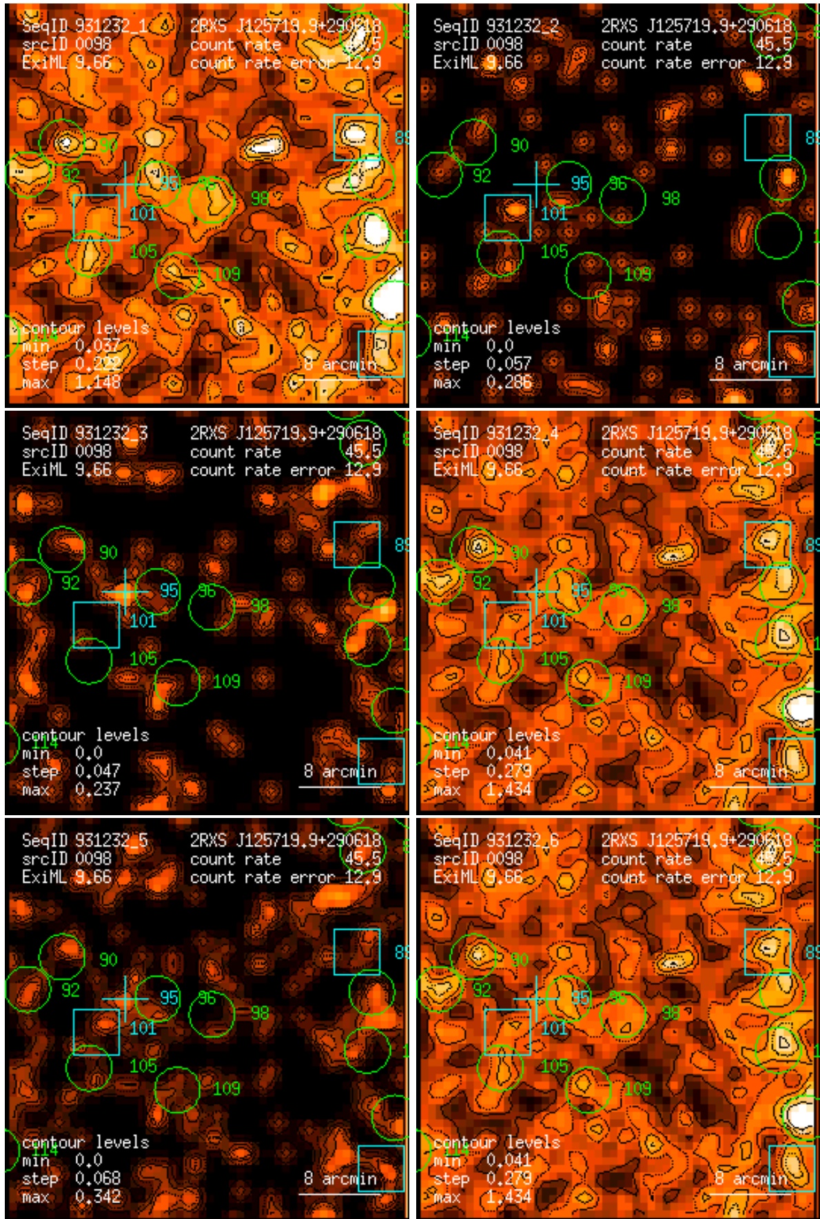
Figure 98: RASS 931232: detection 0098: band rate images, Gaussian filter: (1) PSPC channels 11 – 41, (2) 52 – 90, (3) 91 – 201, (4) 11 – 235, (5) 52 – 201, (6) 11 – 201. Broad band rates in counts/ks. Band rate contour levels in counts/ks/arcmin 2 .
