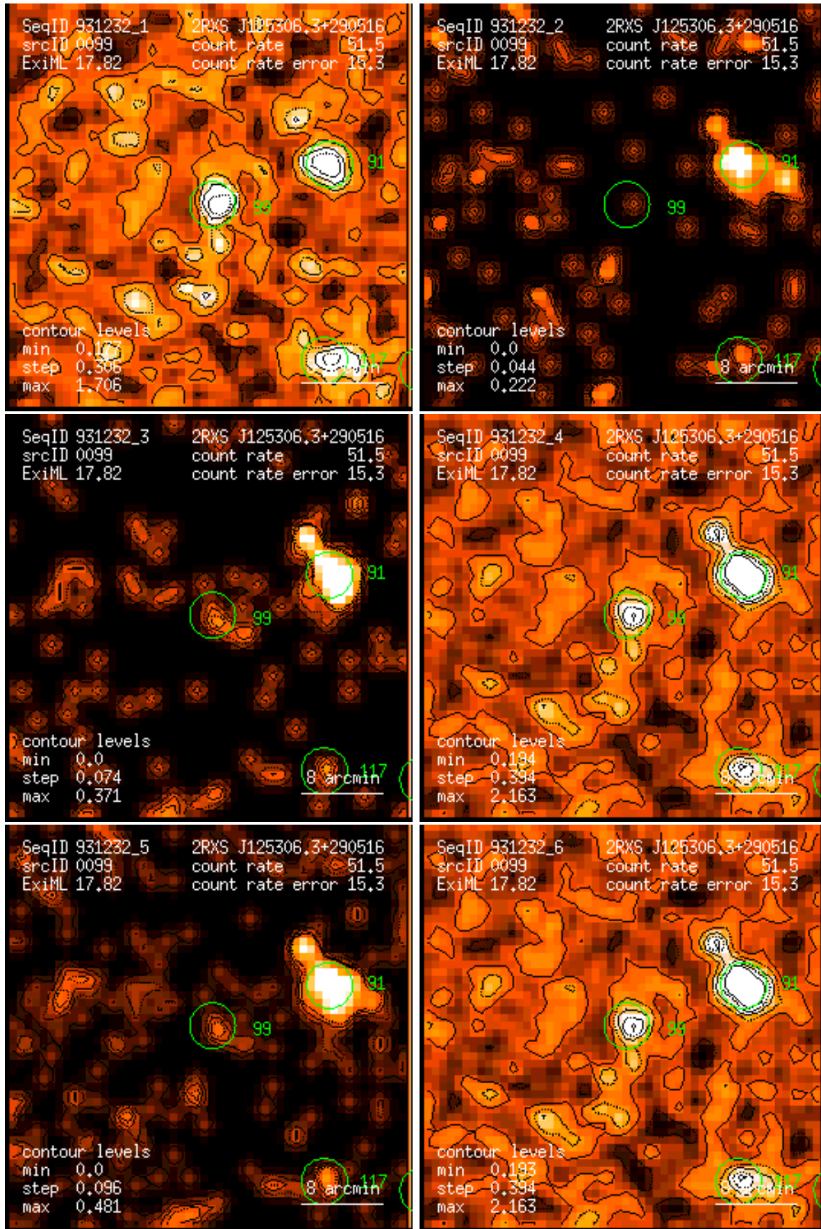
Figure 99: RASS 931232: detection 0099: band rate images, Gaussian filter: (1) PSPC channels 11 – 41, (2) 52 – 90, (3) 91 – 201, (4) 11 – 235, (5) 52 – 201, (6) 11 – 201. Broad band rates in counts/ks. Band rate contour levels in counts/ks/arcmin 2 .
