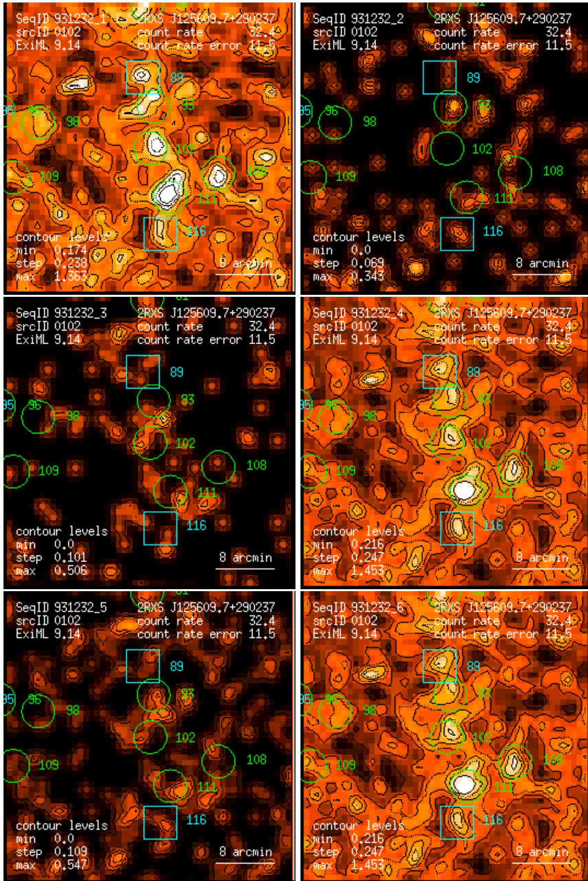
Figure 102: RASS 931232: detection 0102: band rate images, Gaussian filter: (1) PSPC channels 11 – 41, (2) 52 – 90, (3) 91 – 201, (4) 11 – 235, (5) 52 – 201, (6) 11 – 201. Broad band rates in counts/ks. Band rate contour levels in counts/ks/arcmin 2 .
