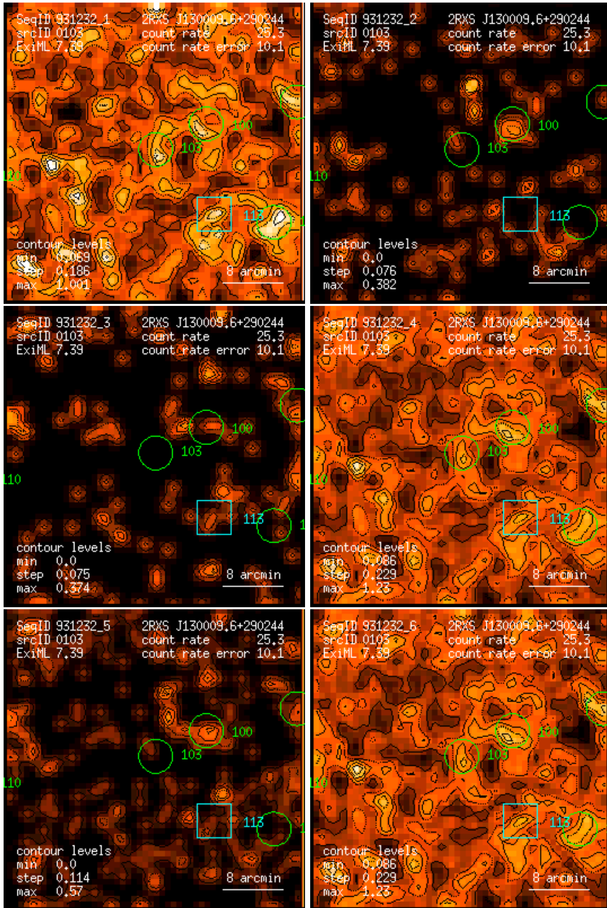
Figure 103: RASS 931232: detection 0103: band rate images, Gaussian filter: (1) PSPC channels 11 – 41, (2) 52 – 90, (3) 91 – 201, (4) 11 – 235, (5) 52 – 201, (6) 11 – 201. Broad band rates in counts/ks. Band rate contour levels in counts/ks/arcmin 2 .
