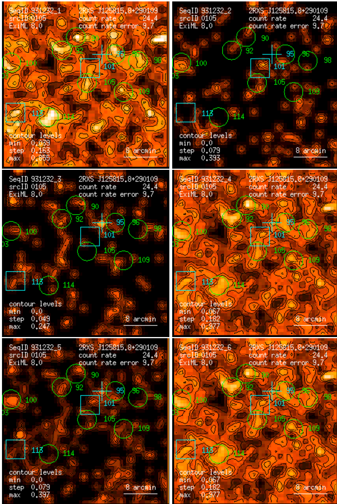
Figure 105: RASS 931232: detection 0105: band rate images, Gaussian filter: (1) PSPC channels 11 – 41, (2) 52 – 90, (3) 91 – 201, (4) 11 – 235, (5) 52 – 201, (6) 11 – 201. Broad band rates in counts/ks. Band rate contour levels in counts/ks/arcmin 2 .
