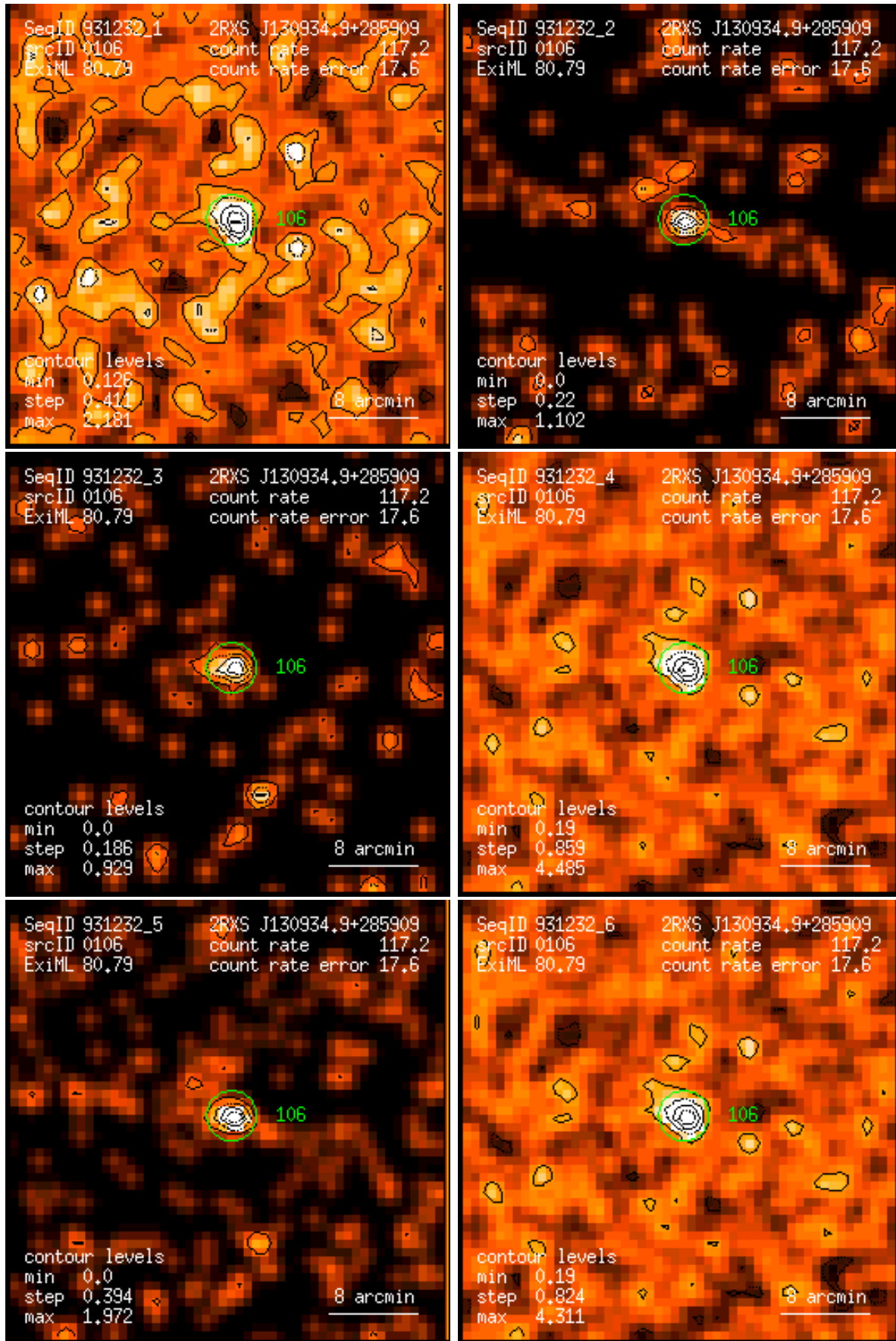
Figure 106: RASS 931232: detection 0106: band rate images, Gaussian filter: (1) PSPC channels 11 – 41, (2) 52 – 90, (3) 91 – 201, (4) 11 – 235, (5) 52 – 201, (6) 11 – 201. Broad band rates in counts/ks. Band rate contour levels in counts/ks/arcmin 2 .
