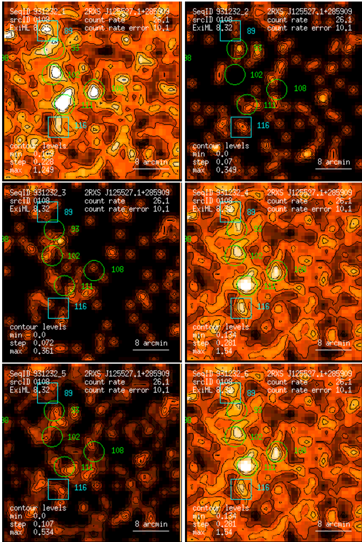
Figure 108: RASS 931232: detection 0108: band rate images, Gaussian filter: (1) PSPC channels 11 – 41, (2) 52 – 90, (3) 91 – 201, (4) 11 – 235, (5) 52 – 201, (6) 11 – 201. Broad band rates in counts/ks. Band rate contour levels in counts/ks/arcmin 2 .
