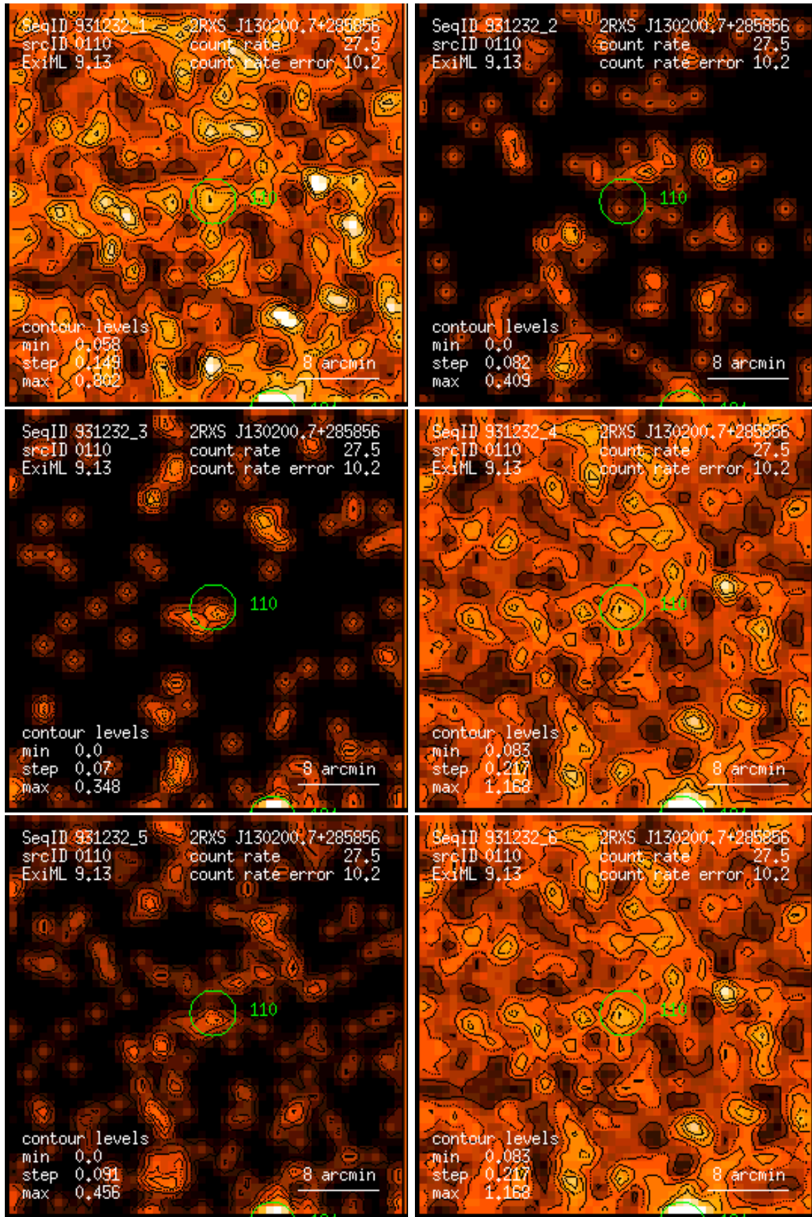
Figure 110: RASS 931232: detection 0110: band rate images, Gaussian filter: (1) PSPC channels 11 – 41, (2) 52 – 90, (3) 91 – 201, (4) 11 – 235, (5) 52 – 201, (6) 11 – 201. Broad band rates in counts/ks. Band rate contour levels in counts/ks/arcmin 2 .
