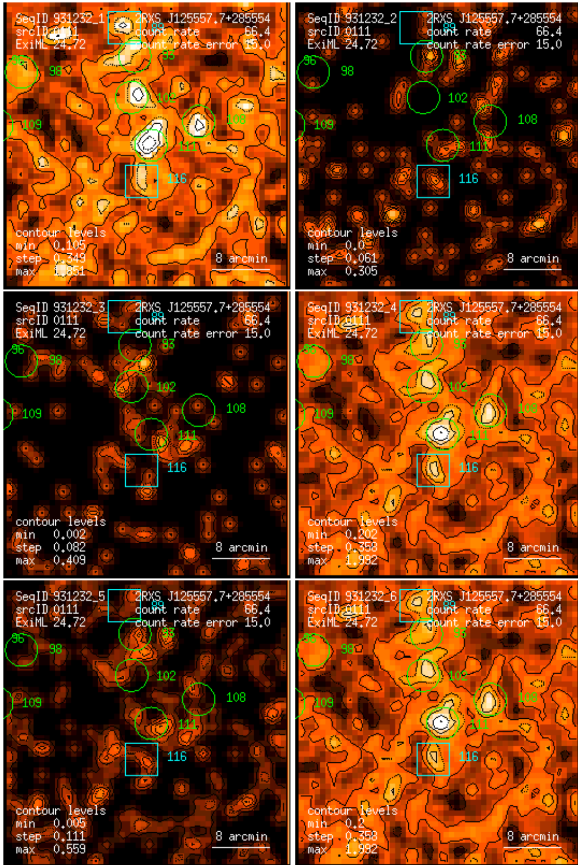
Figure 111: RASS 931232: detection 0111: band rate images, Gaussian filter: (1) PSPC channels 11 – 41, (2) 52 – 90, (3) 91 – 201, (4) 11 – 235, (5) 52 – 201, (6) 11 – 201. Broad band rates in counts/ks. Band rate contour levels in counts/ks/arcmin 2 .
