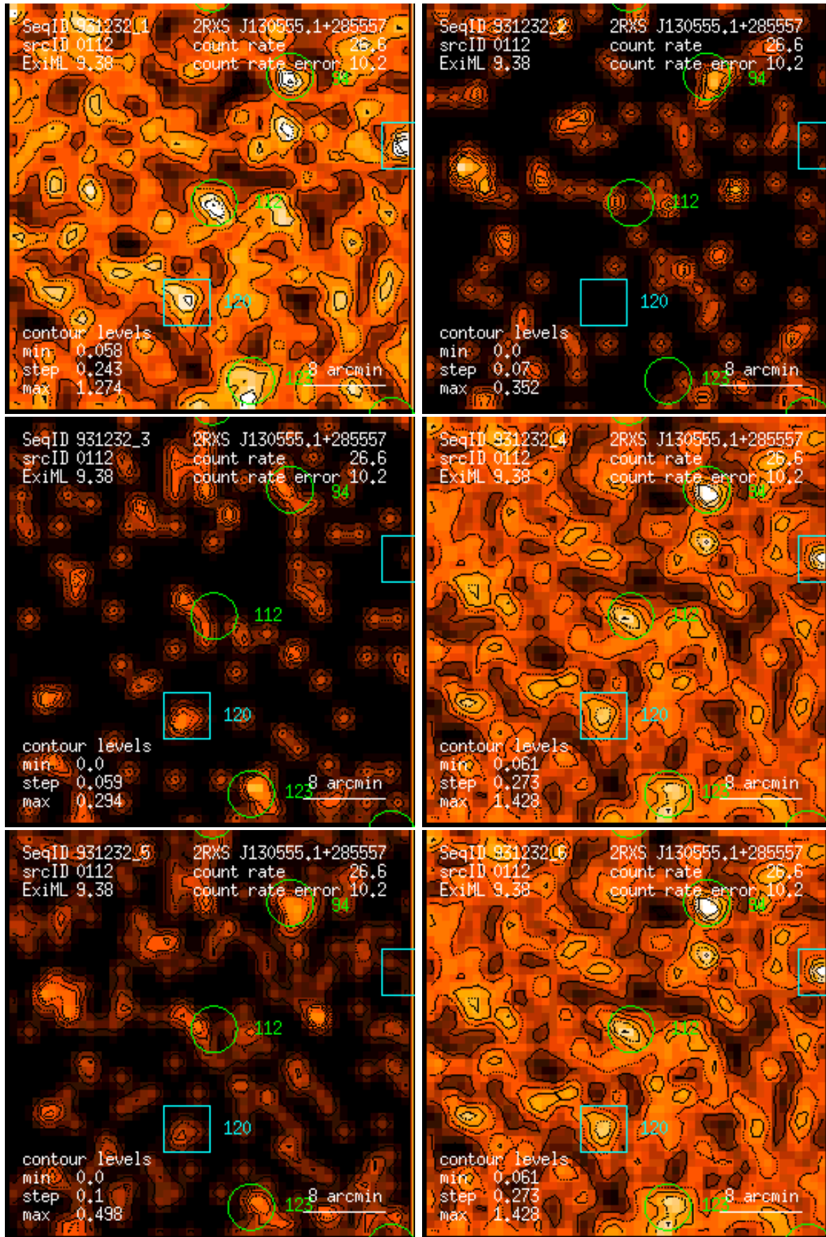
Figure 112: RASS 931232: detection 0112: band rate images, Gaussian filter: (1) PSPC channels 11 – 41, (2) 52 – 90, (3) 91 – 201, (4) 11 – 235, (5) 52 – 201, (6) 11 – 201. Broad band rates in counts/ks. Band rate contour levels in counts/ks/arcmin 2 .
