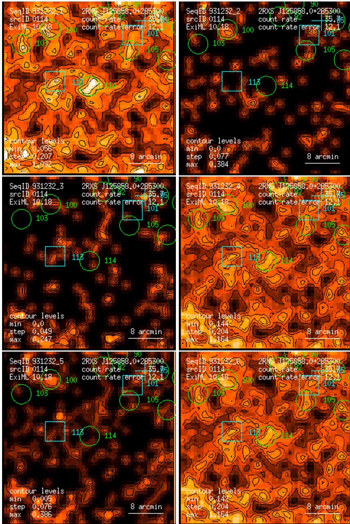
Figure 114: RASS 931232: detection 0114: band rate images, Gaussian filter: (1) PSPC channels 11 – 41, (2) 52 – 90, (3) 91 – 201, (4) 11 – 235, (5) 52 – 201, (6) 11 – 201. Broad band rates in counts/ks. Band rate contour levels in counts/ks/arcmin 2 .
