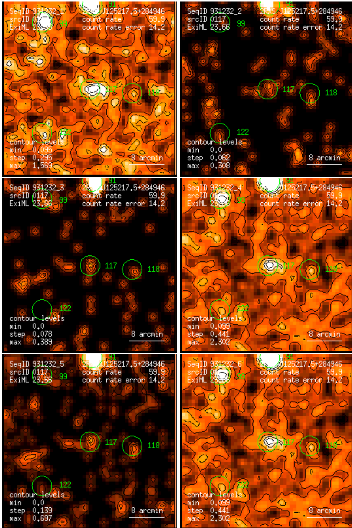
Figure 117: RASS 931232: detection 0117: band rate images, Gaussian filter: (1) PSPC channels 11 – 41, (2) 52 – 90, (3) 91 – 201, (4) 11 – 235, (5) 52 – 201, (6) 11 – 201. Broad band rates in counts/ks. Band rate contour levels in counts/ks/arcmin 2 .
