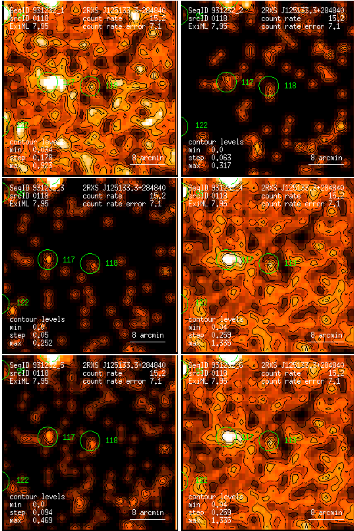
Figure 118: RASS 931232: detection 0118: band rate images, Gaussian filter: (1) PSPC channels 11 – 41, (2) 52 – 90, (3) 91 – 201, (4) 11 – 235, (5) 52 – 201, (6) 11 – 201. Broad band rates in counts/ks. Band rate contour levels in counts/ks/arcmin 2 .
