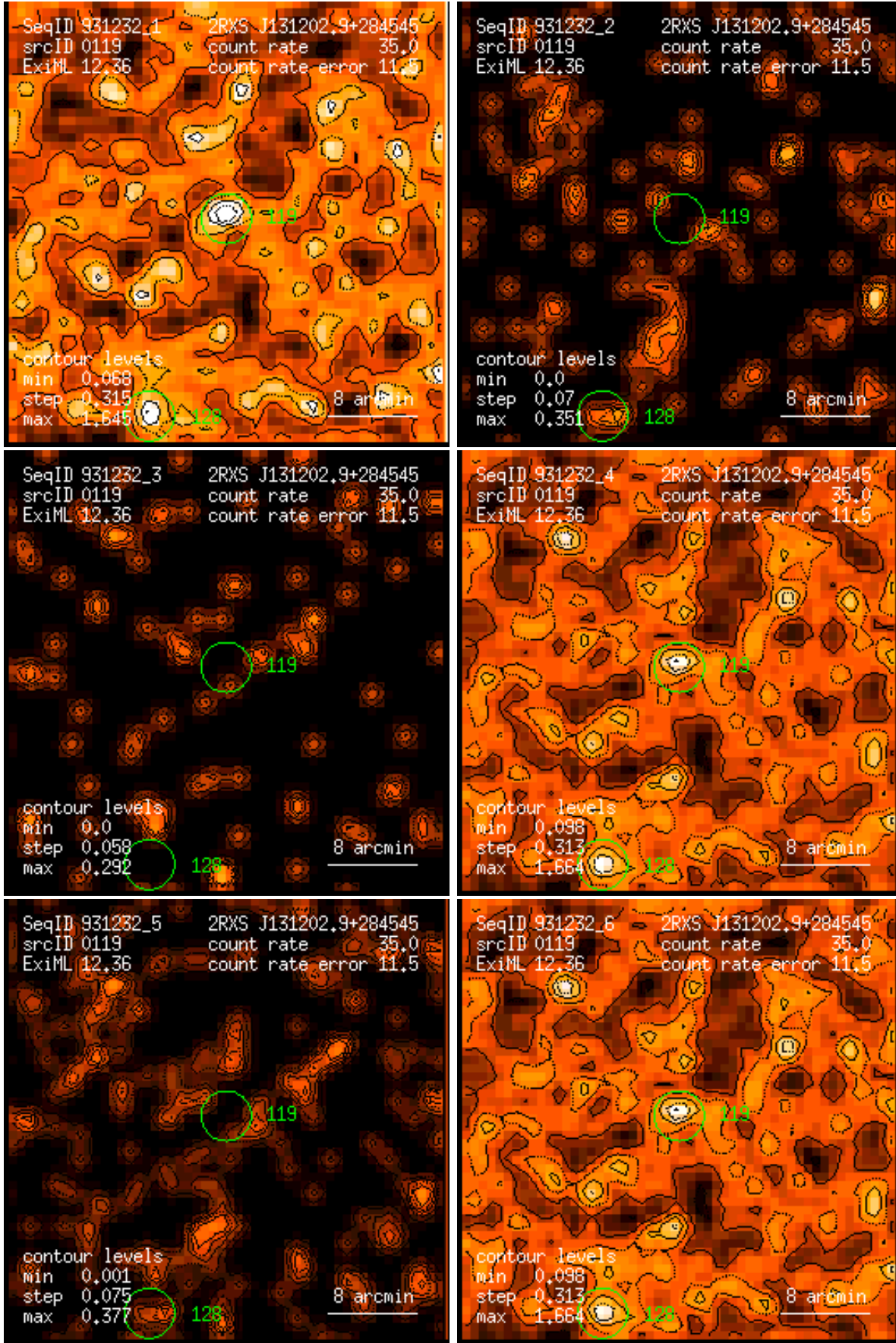
Figure 119: RASS 931232: detection 0119: band rate images, Gaussian filter: (1) PSPC channels 11 – 41, (2) 52 – 90, (3) 91 – 201, (4) 11 – 235, (5) 52 – 201, (6) 11 – 201. Broad band rates in counts/ks. Band rate contour levels in counts/ks/arcmin 2 .
