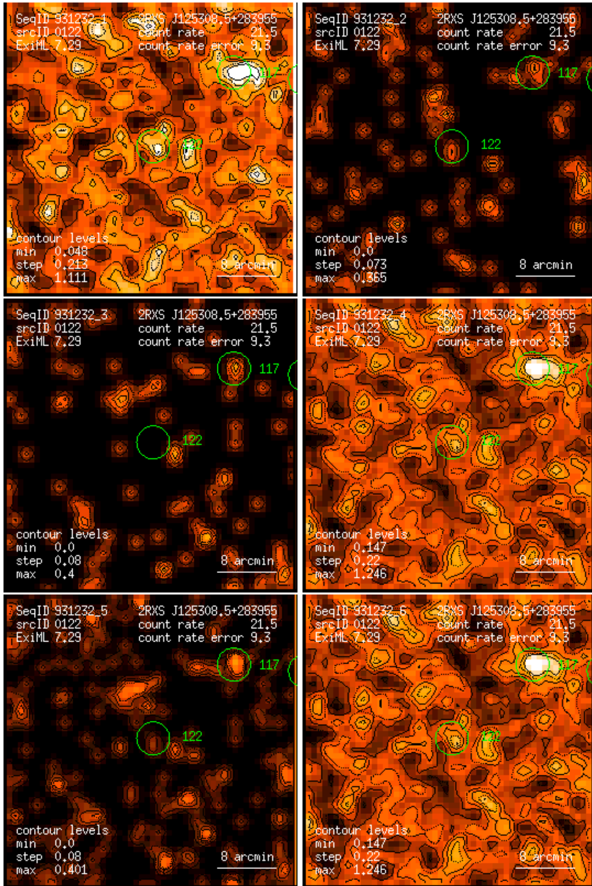
Figure 122: RASS 931232: detection 0122: band rate images, Gaussian filter: (1) PSPC channels 11 – 41, (2) 52 – 90, (3) 91 – 201, (4) 11 – 235, (5) 52 – 201, (6) 11 – 201. Broad band rates in counts/ks. Band rate contour levels in counts/ks/arcmin 2 .
