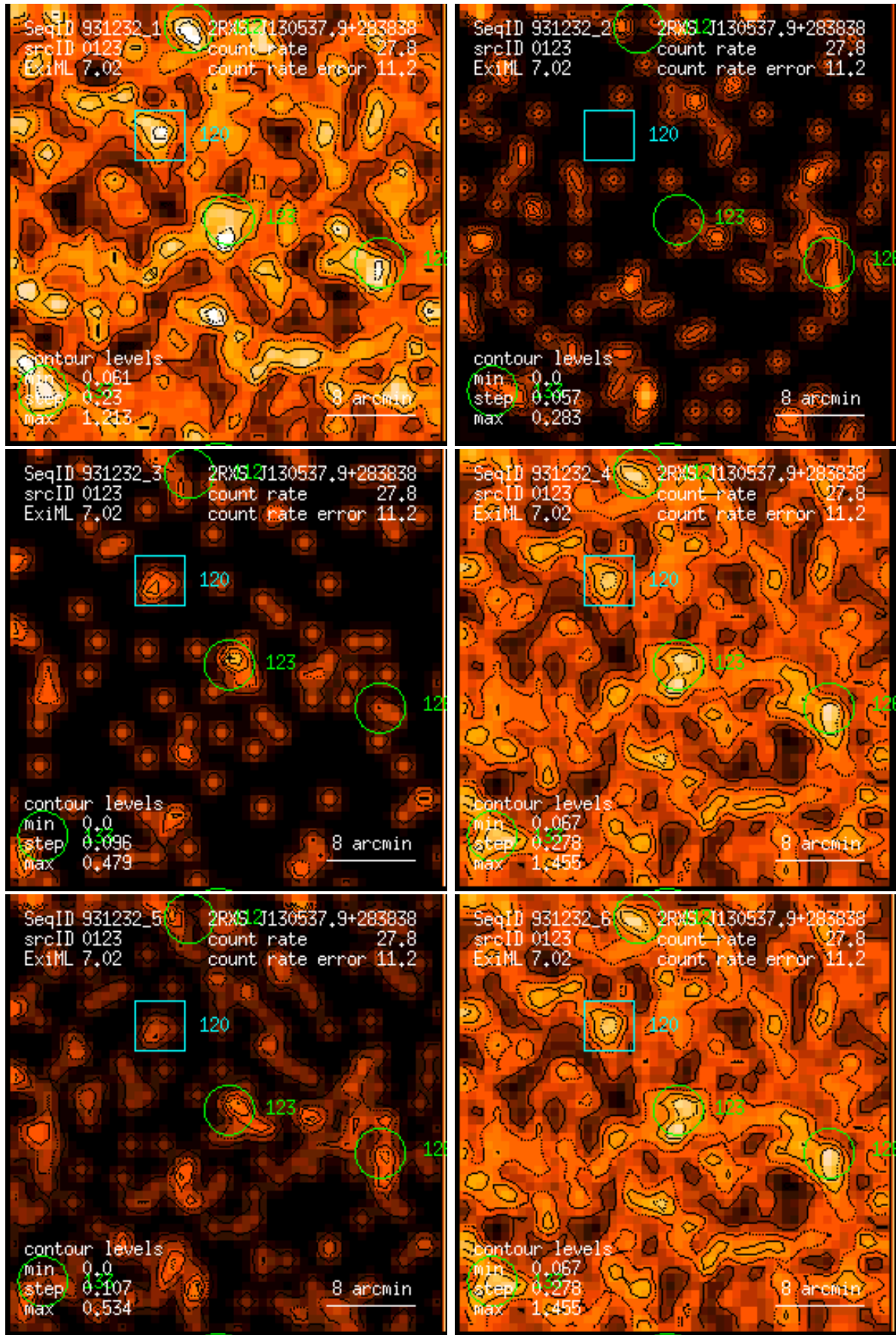
Figure 123: RASS 931232: detection 0123: band rate images, Gaussian filter: (1) PSPC channels 11 – 41, (2) 52 – 90, (3) 91 – 201, (4) 11 – 235, (5) 52 – 201, (6) 11 – 201. Broad band rates in counts/ks. Band rate contour levels in counts/ks/arcmin 2 .
