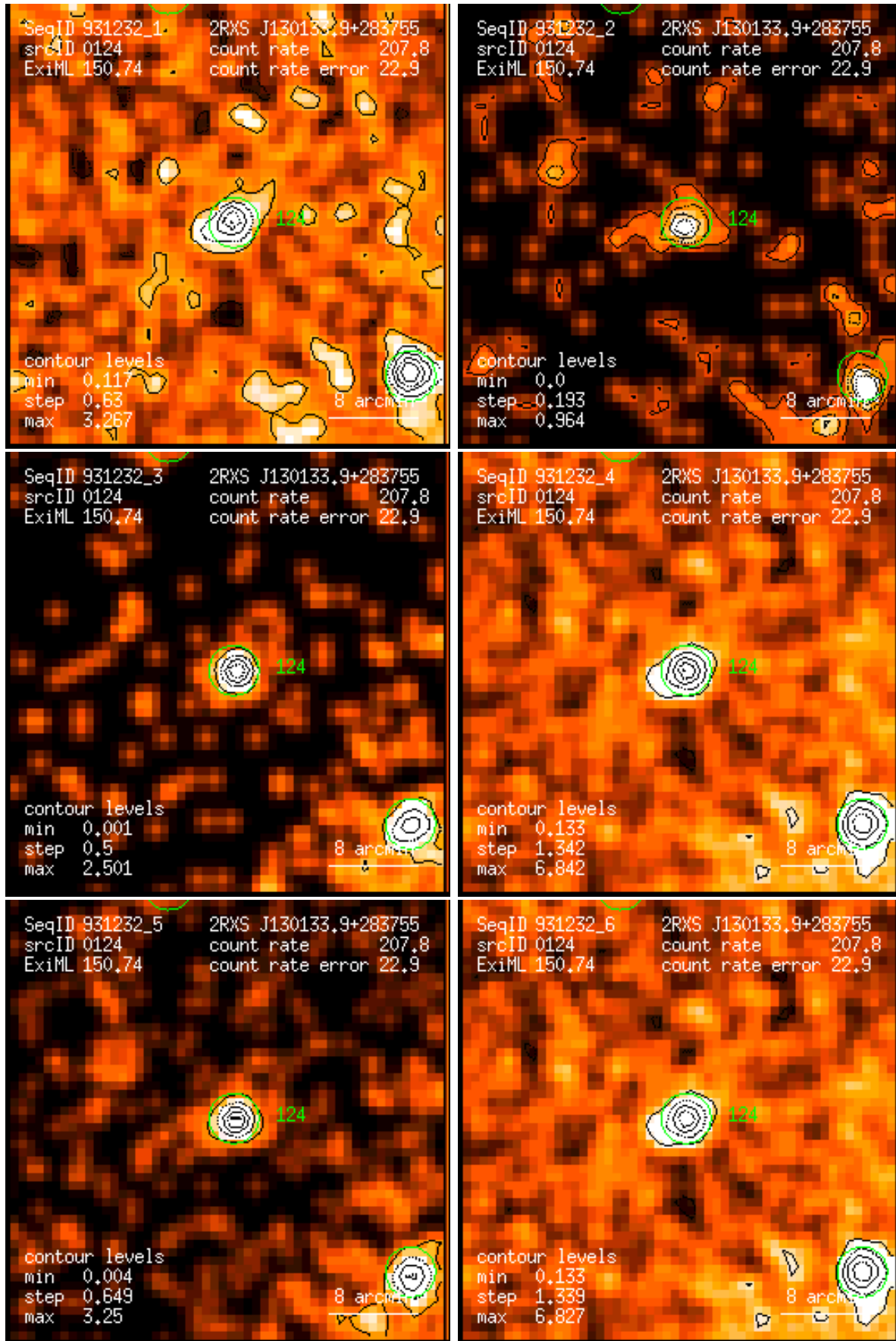
Figure 124: RASS 931232: detection 0124: band rate images, Gaussian filter: (1) PSPC channels 11 – 41, (2) 52 – 90, (3) 91 – 201, (4) 11 – 235, (5) 52 – 201, (6) 11 – 201. Broad band rates in counts/ks. Band rate contour levels in counts/ks/arcmin 2 .
