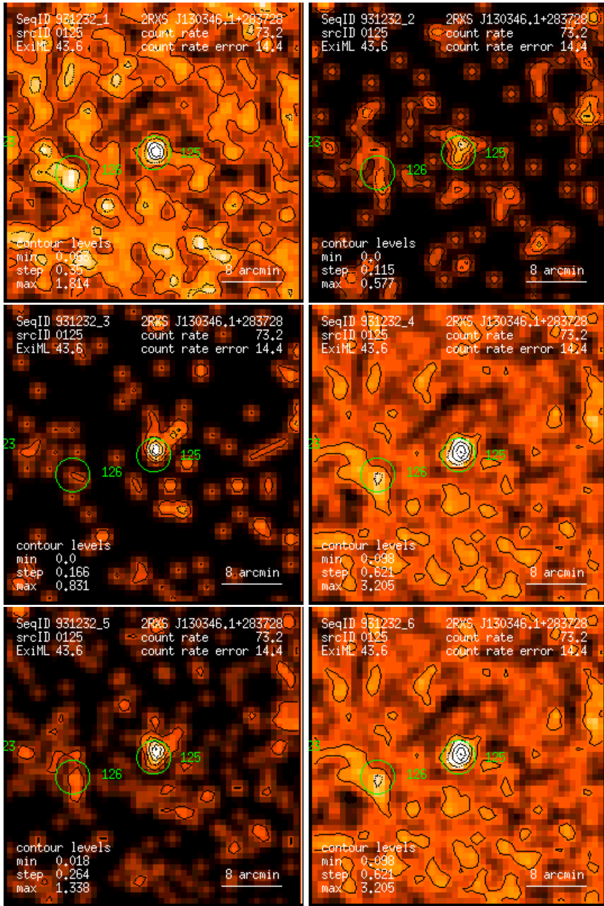
Figure 125: RASS 931232: detection 0125: band rate images, Gaussian filter: (1) PSPC channels 11 – 41, (2) 52 – 90, (3) 91 – 201, (4) 11 – 235, (5) 52 – 201, (6) 11 – 201. Broad band rates in counts/ks. Band rate contour levels in counts/ks/arcmin 2 .
