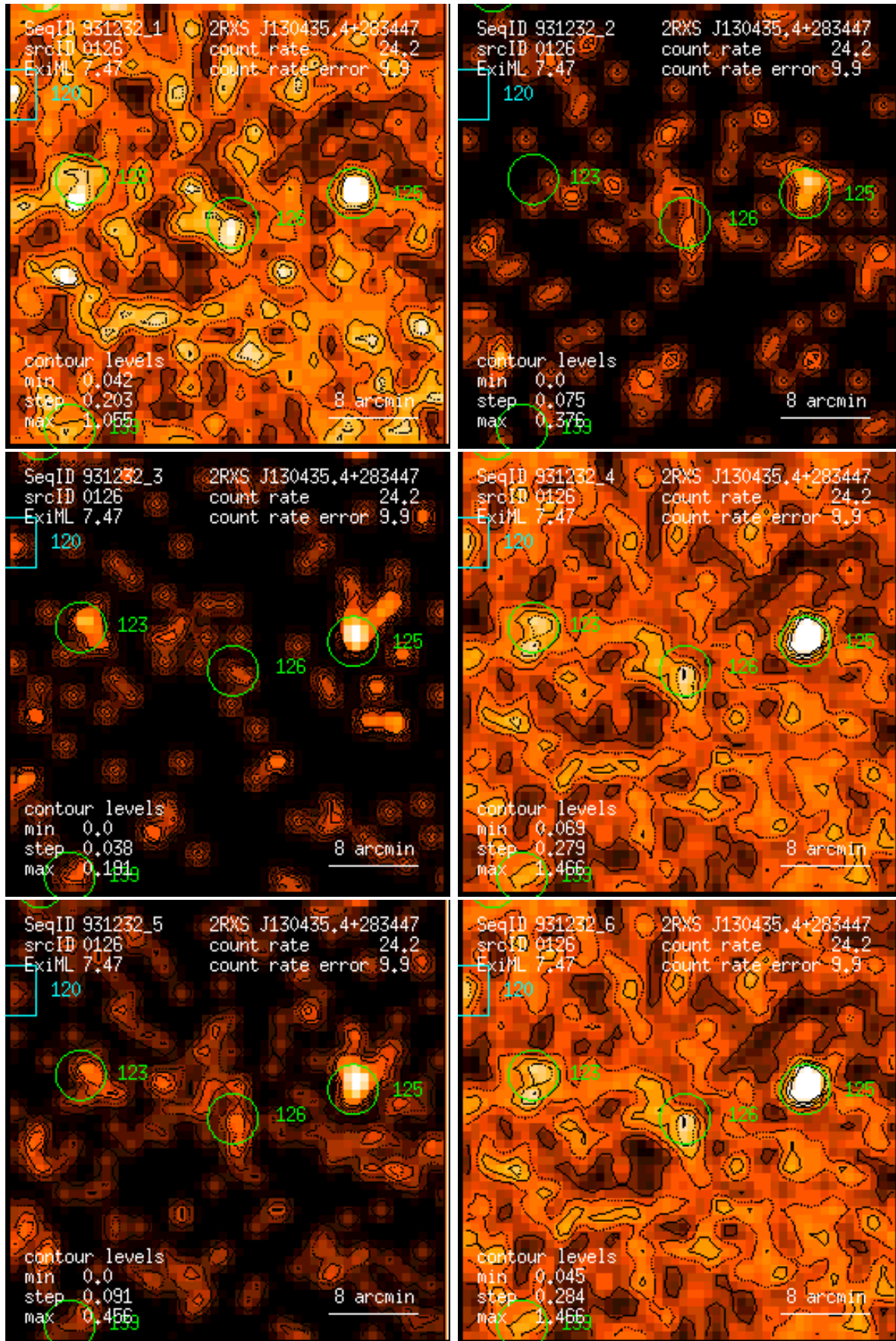
Figure 126: RASS 931232: detection 0126: band rate images, Gaussian filter: (1) PSPC channels 11 – 41, (2) 52 – 90, (3) 91 – 201, (4) 11 – 235, (5) 52 – 201, (6) 11 – 201. Broad band rates in counts/ks. Band rate contour levels in counts/ks/arcmin 2 .
