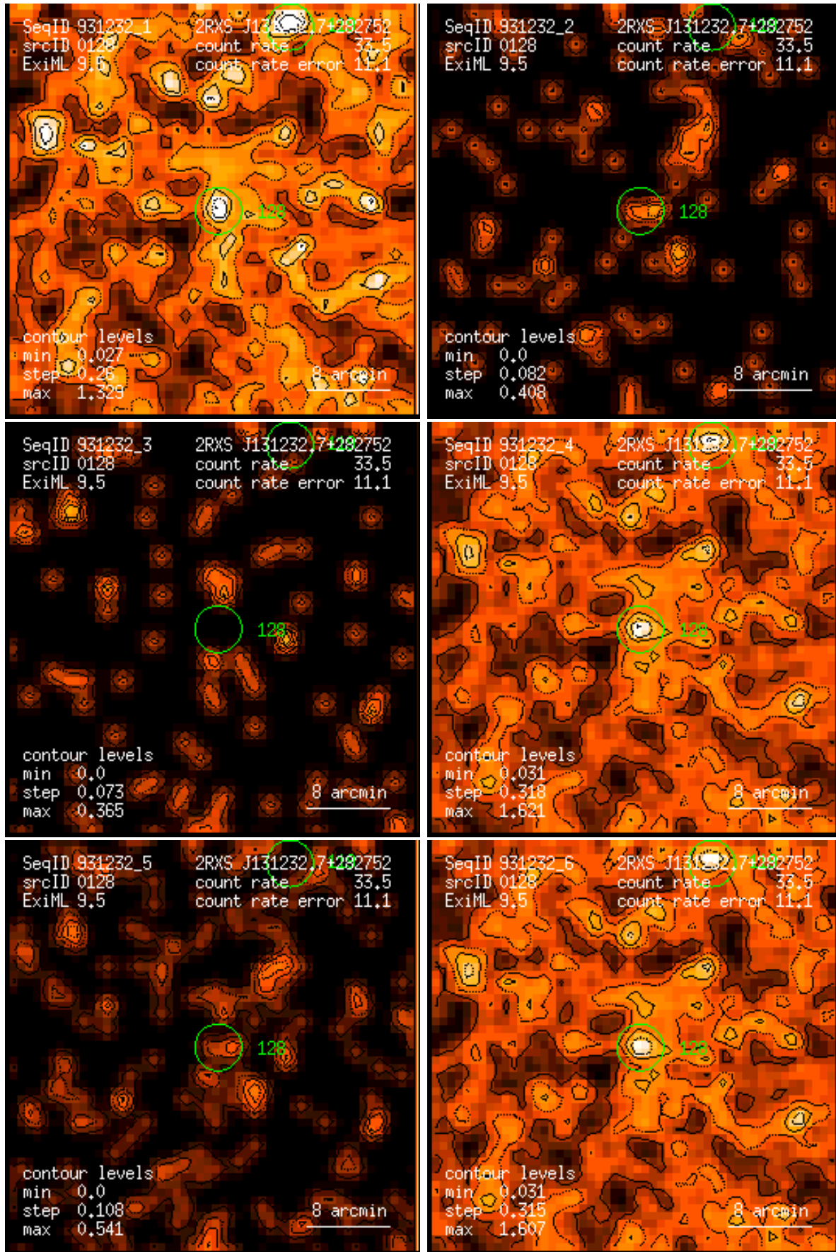
Figure 128: RASS 931232: detection 0128: band rate images, Gaussian filter: (1) PSPC channels 11 – 41, (2) 52 – 90, (3) 91 – 201, (4) 11 – 235, (5) 52 – 201, (6) 11 – 201. Broad band rates in counts/ks. Band rate contour levels in counts/ks/arcmin 2 .
