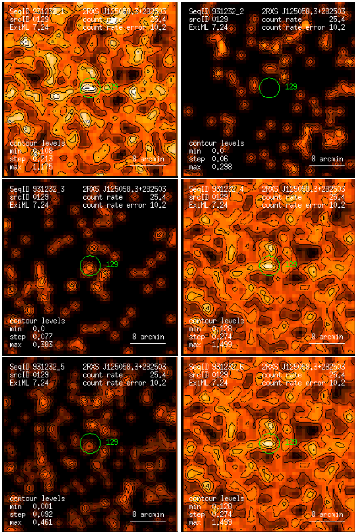
Figure 129: RASS 931232: detection 0129: band rate images, Gaussian filter: (1) PSPC channels 11 – 41, (2) 52 – 90, (3) 91 – 201, (4) 11 – 235, (5) 52 – 201, (6) 11 – 201. Broad band rates in counts/ks. Band rate contour levels in counts/ks/arcmin 2 .
