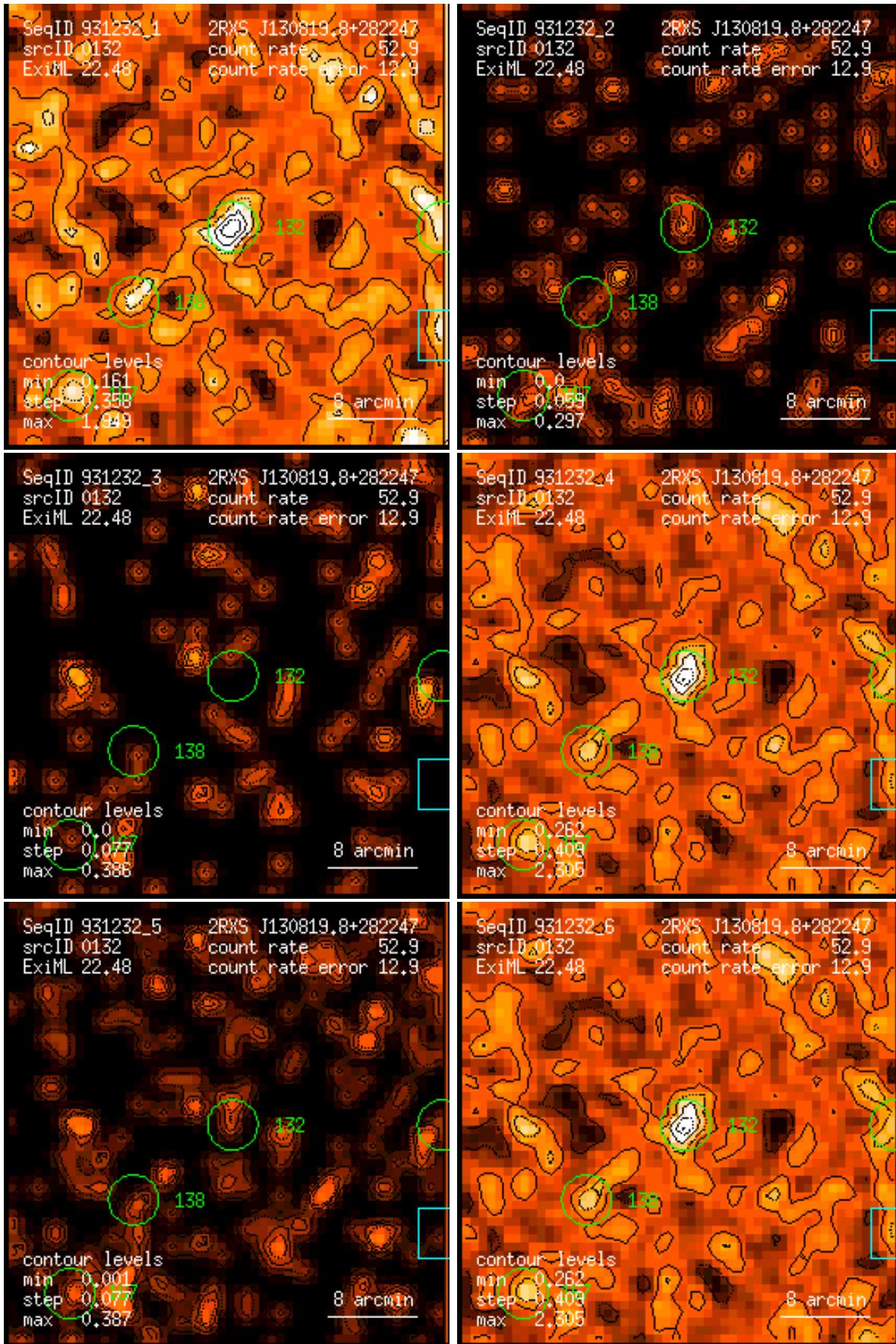
Figure 132: RASS 931232: detection 0132: band rate images, Gaussian filter: (1) PSPC channels 11 – 41, (2) 52 – 90, (3) 91 – 201, (4) 11 – 235, (5) 52 – 201, (6) 11 – 201. Broad band rates in counts/ks. Band rate contour levels in counts/ks/arcmin 2 .
