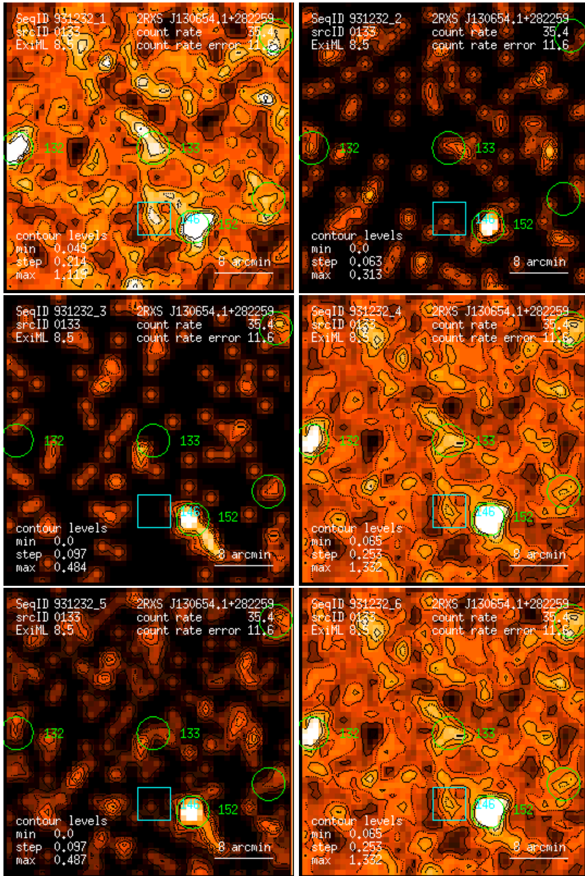
Figure 133: RASS 931232: detection 0133: band rate images, Gaussian filter: (1) PSPC channels 11 – 41, (2) 52 – 90, (3) 91 – 201, (4) 11 – 235, (5) 52 – 201, (6) 11 – 201. Broad band rates in counts/ks. Band rate contour levels in counts/ks/arcmin 2 .
