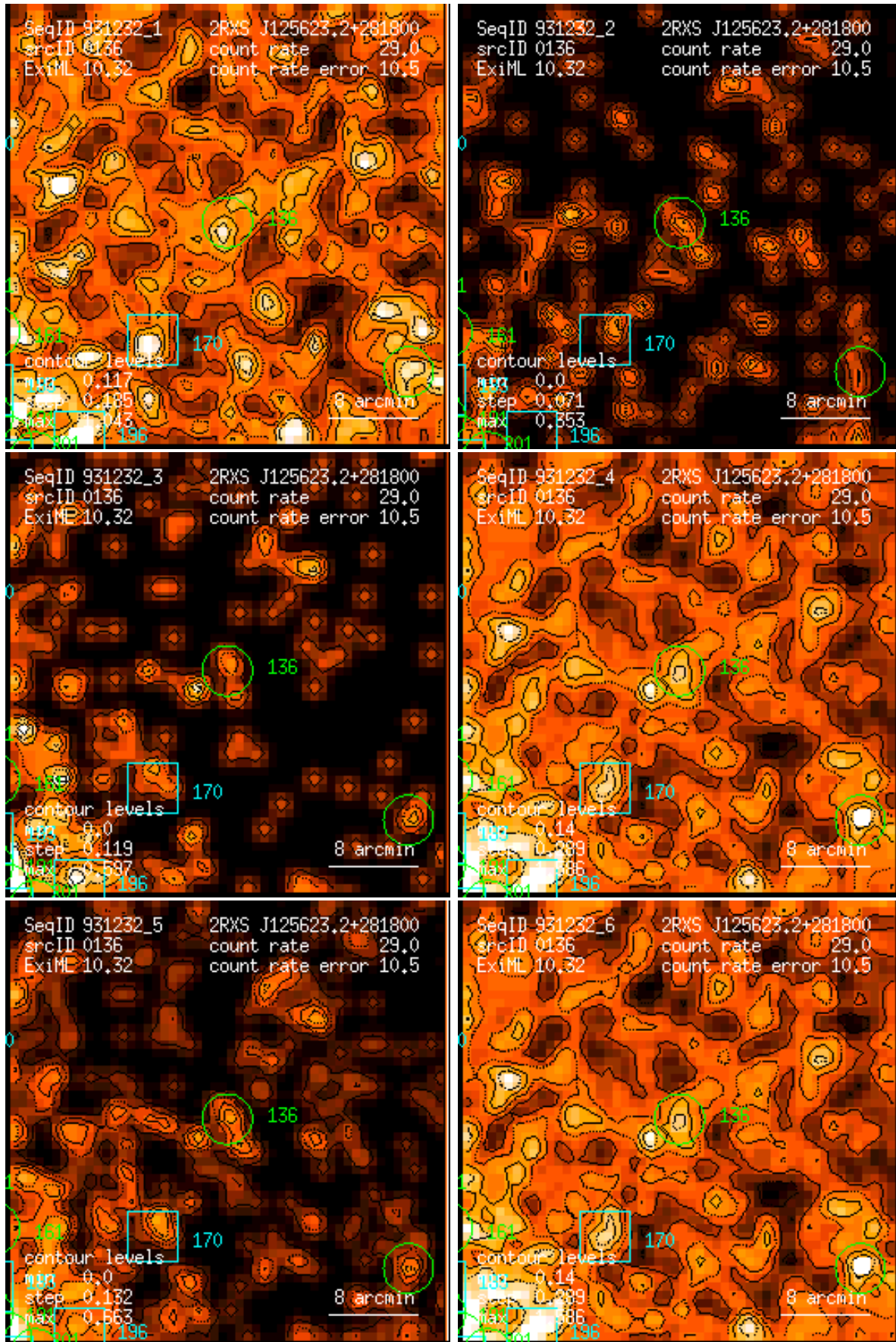
Figure 136: RASS 931232: detection 0136: band rate images, Gaussian filter: (1) PSPC channels 11 – 41, (2) 52 – 90, (3) 91 – 201, (4) 11 – 235, (5) 52 – 201, (6) 11 – 201. Broad band rates in counts/ks. Band rate contour levels in counts/ks/arcmin 2 .
