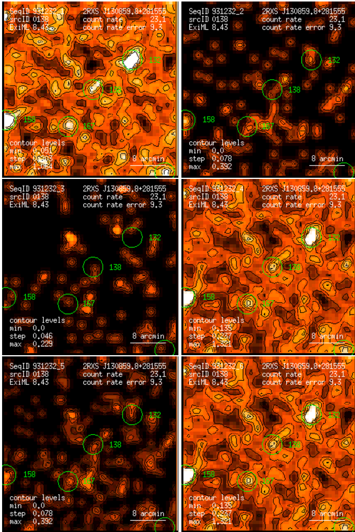
Figure 138: RASS 931232: detection 0138: band rate images, Gaussian filter: (1) PSPC channels 11 – 41, (2) 52 – 90, (3) 91 – 201, (4) 11 – 235, (5) 52 – 201, (6) 11 – 201. Broad band rates in counts/ks. Band rate contour levels in counts/ks/arcmin 2 .
