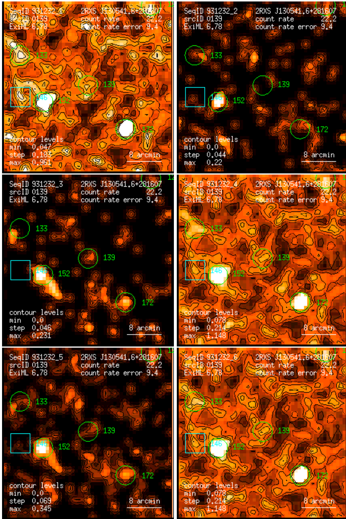
Figure 139: RASS 931232: detection 0139: band rate images, Gaussian filter: (1) PSPC channels 11 – 41, (2) 52 – 90, (3) 91 – 201, (4) 11 – 235, (5) 52 – 201, (6) 11 – 201. Broad band rates in counts/ks. Band rate contour levels in counts/ks/arcmin 2 .
