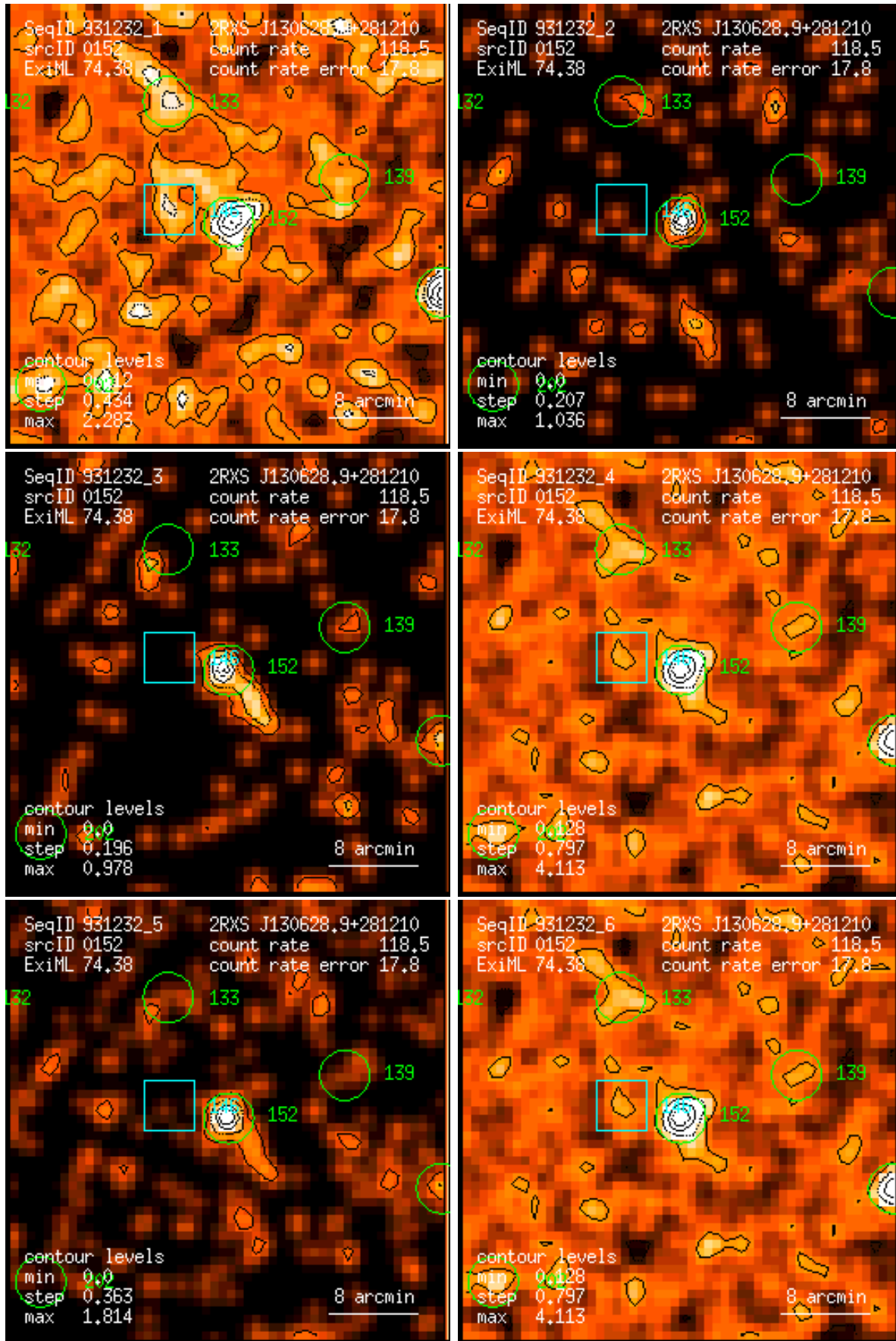
Figure 152: RASS 931232: detection 0152: band rate images, Gaussian filter: (1) PSPC channels 11 – 41, (2) 52 – 90, (3) 91 – 201, (4) 11 – 235, (5) 52 – 201, (6) 11 – 201. Broad band rates in counts/ks. Band rate contour levels in counts/ks/arcmin 2 .
