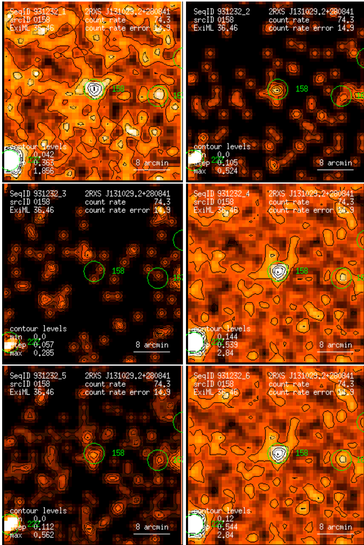
Figure 158: RASS 931232: detection 0158: band rate images, Gaussian filter: (1) PSPC channels 11 – 41, (2) 52 – 90, (3) 91 – 201, (4) 11 – 235, (5) 52 – 201, (6) 11 – 201. Broad band rates in counts/ks. Band rate contour levels in counts/ks/arcmin 2 .
