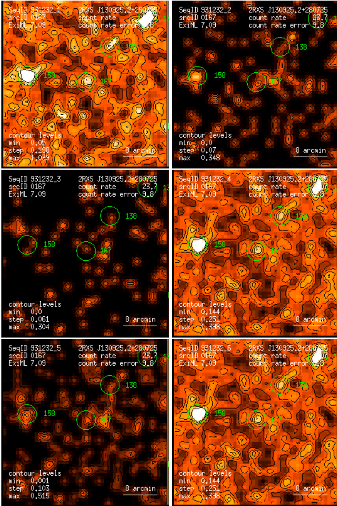
Figure 167: RASS 931232: detection 0167: band rate images, Gaussian filter: (1) PSPC channels 11 – 41, (2) 52 – 90, (3) 91 – 201, (4) 11 – 235, (5) 52 – 201, (6) 11 – 201. Broad band rates in counts/ks. Band rate contour levels in counts/ks/arcmin 2 .
