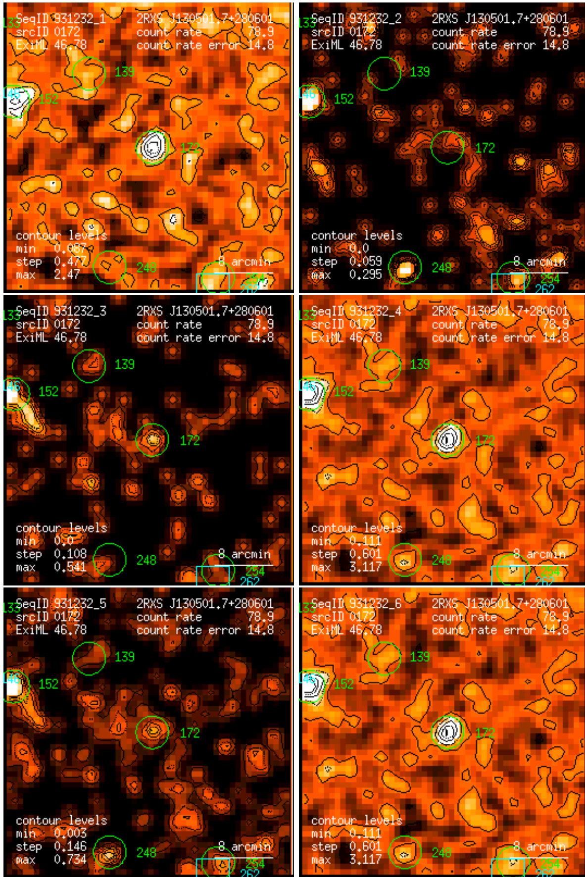
Figure 172: RASS 931232: detection 0172: band rate images, Gaussian filter: (1) PSPC channels 11 – 41, (2) 52 – 90, (3) 91 – 201, (4) 11 – 235, (5) 52 – 201, (6) 11 – 201. Broad band rates in counts/ks. Band rate contour levels in counts/ks/arcmin 2 .
