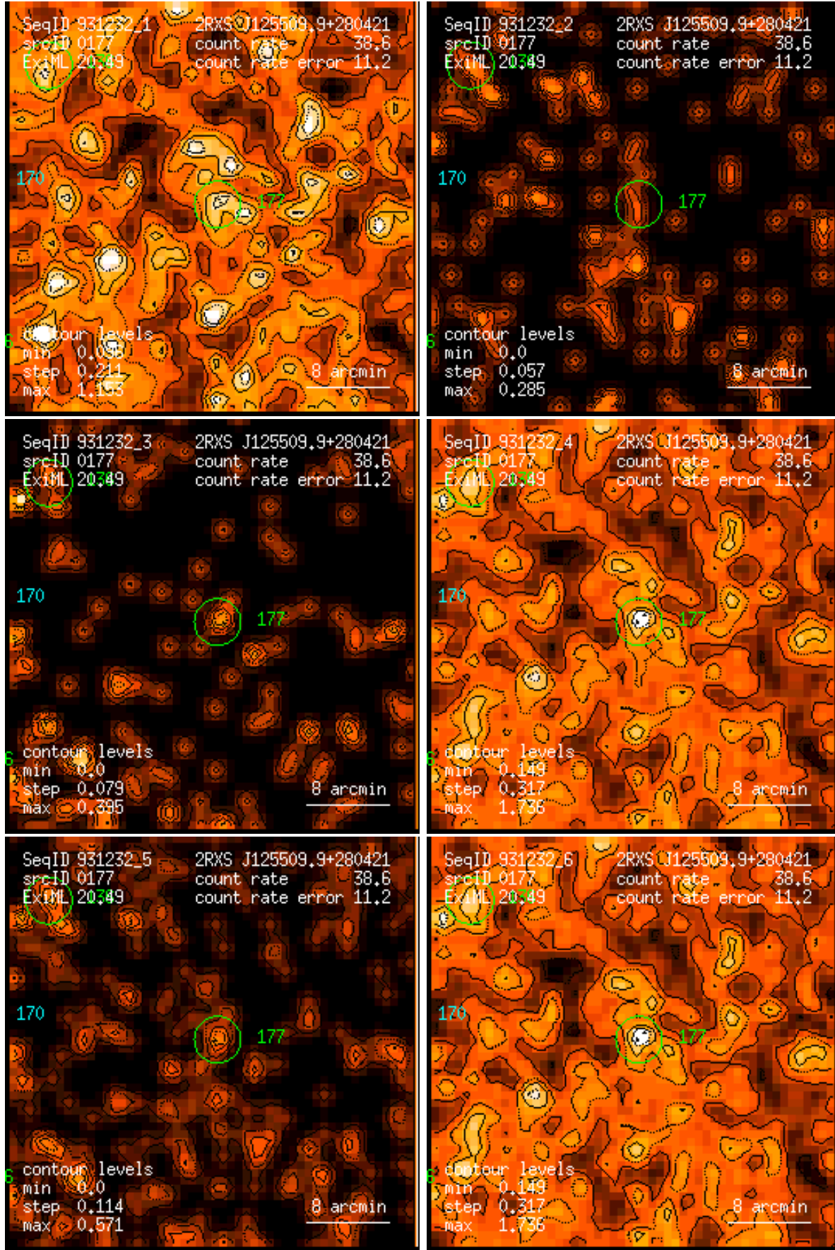
Figure 177: RASS 931232: detection 0177: band rate images, Gaussian filter: (1) PSPC channels 11 – 41, (2) 52 – 90, (3) 91 – 201, (4) 11 – 235, (5) 52 – 201, (6) 11 – 201. Broad band rates in counts/ks. Band rate contour levels in counts/ks/arcmin 2 .
