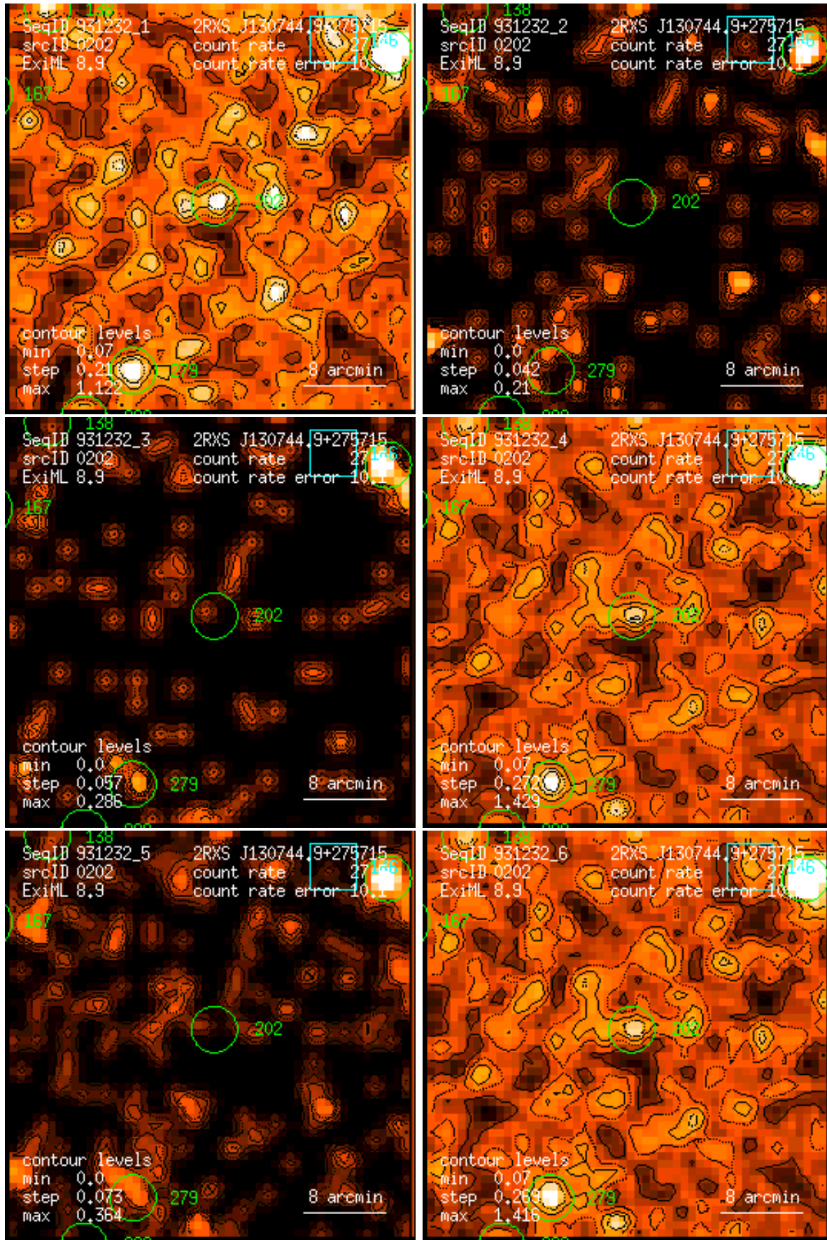
Figure 202: RASS 931232: detection 0202: band rate images, Gaussian filter: (1) PSPC channels 11 – 41, (2) 52 – 90, (3) 91 – 201, (4) 11 – 235, (5) 52 – 201, (6) 11 – 201. Broad band rates in counts/ks. Band rate contour levels in counts/ks/arcmin 2 .
