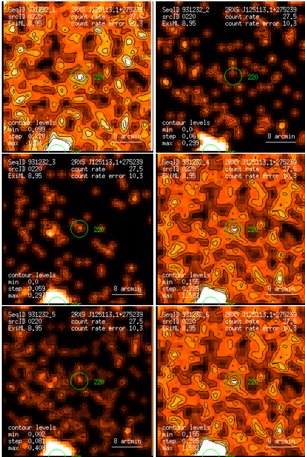
Figure 220: RASS 931232: detection 0220: band rate images, Gaussian filter: (1) PSPC channels 11 – 41, (2) 52 – 90, (3) 91 – 201, (4) 11 – 235, (5) 52 – 201, (6) 11 – 201. Broad band rates in counts/ks. Band rate contour levels in counts/ks/arcmin 2 .
