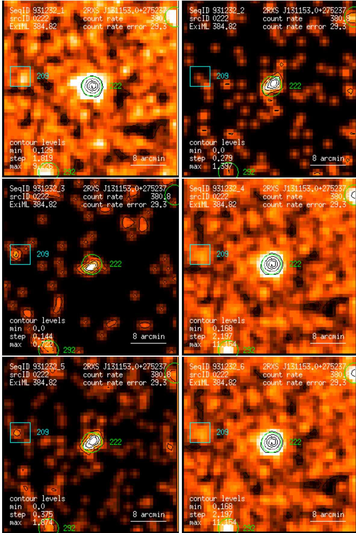
Figure 222: RASS 931232: detection 0222: band rate images, Gaussian filter: (1) PSPC channels 11 – 41, (2) 52 – 90, (3) 91 – 201, (4) 11 – 235, (5) 52 – 201, (6) 11 – 201. Broad band rates in counts/ks. Band rate contour levels in counts/ks/arcmin 2 .
