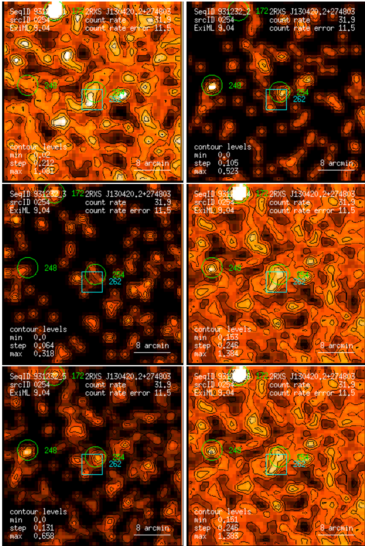
Figure 254: RASS 931232: detection 0254: band rate images, Gaussian filter: (1) PSPC channels 11 – 41, (2) 52 – 90, (3) 91 – 201, (4) 11 – 235, (5) 52 – 201, (6) 11 – 201. Broad band rates in counts/ks. Band rate contour levels in counts/ks/arcmin 2 .
