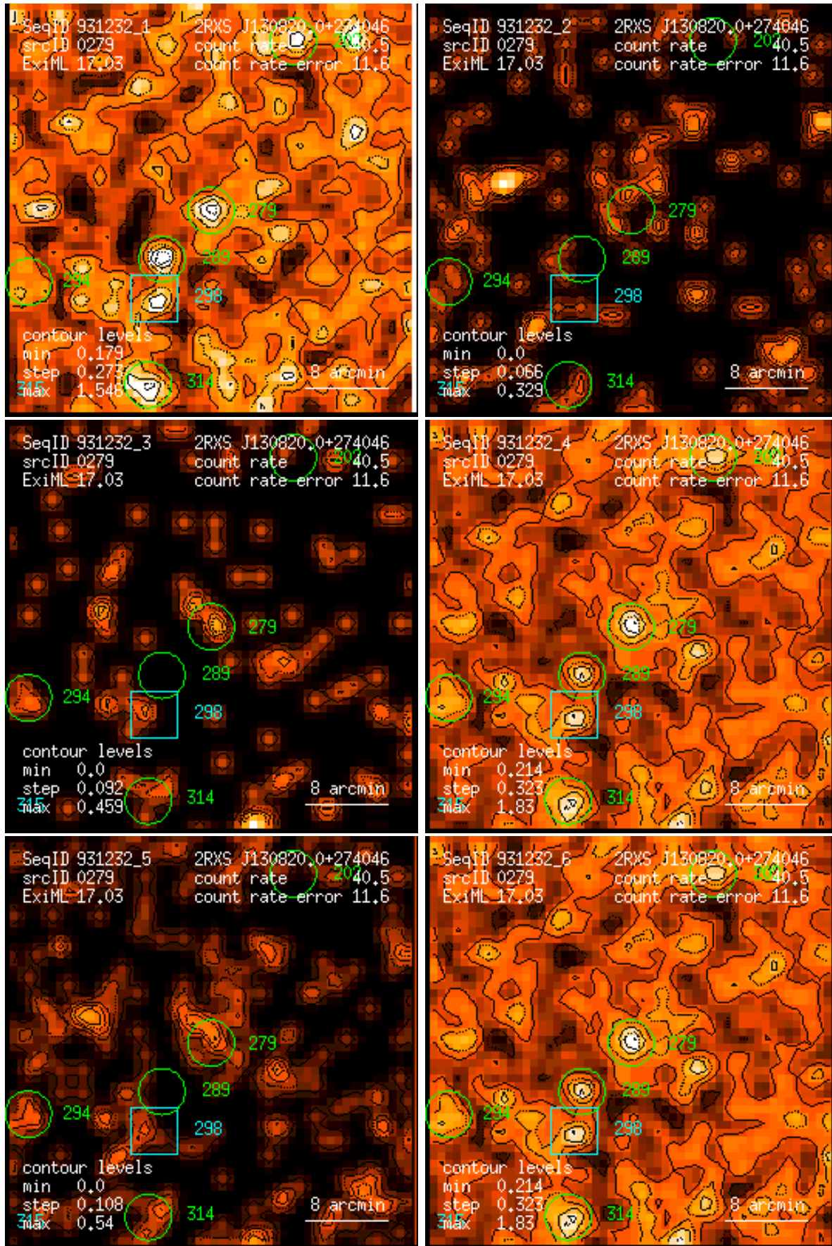
Figure 279: RASS 931232: detection 0279: band rate images, Gaussian filter: (1) PSPC channels 11 – 41, (2) 52 – 90, (3) 91 – 201, (4) 11 – 235, (5) 52 – 201, (6) 11 – 201. Broad band rates in counts/ks. Band rate contour levels in counts/ks/arcmin 2 .
