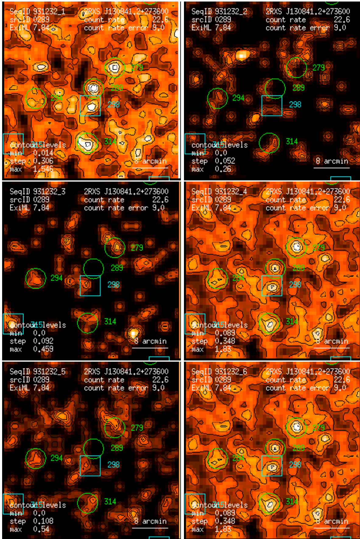
Figure 289: RASS 931232: detection 0289: band rate images, Gaussian filter: (1) PSPC channels 11 – 41, (2) 52 – 90, (3) 91 – 201, (4) 11 – 235, (5) 52 – 201, (6) 11 – 201. Broad band rates in counts/ks. Band rate contour levels in counts/ks/arcmin 2 .
