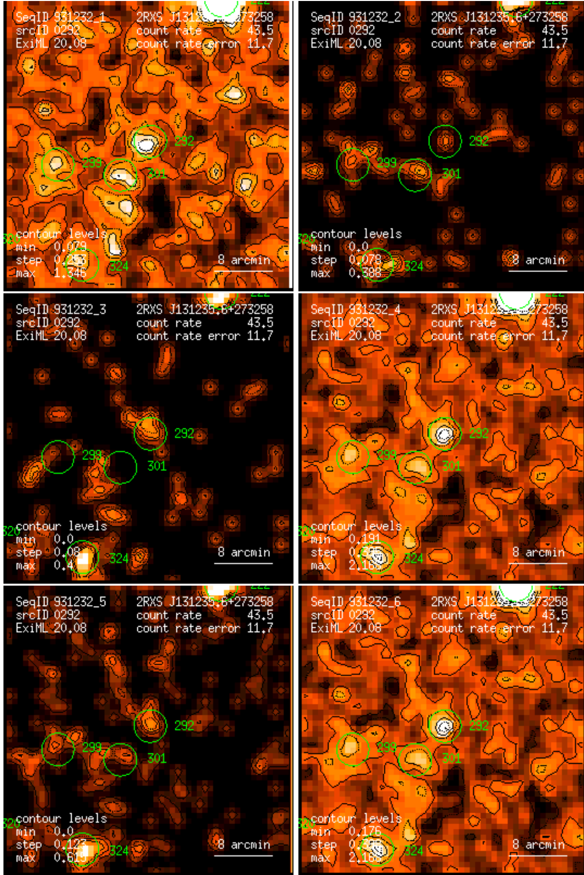
Figure 292: RASS 931232: detection 0292: band rate images, Gaussian filter: (1) PSPC channels 11 – 41, (2) 52 – 90, (3) 91 – 201, (4) 11 – 235, (5) 52 – 201, (6) 11 – 201. Broad band rates in counts/ks. Band rate contour levels in counts/ks/arcmin 2 .
