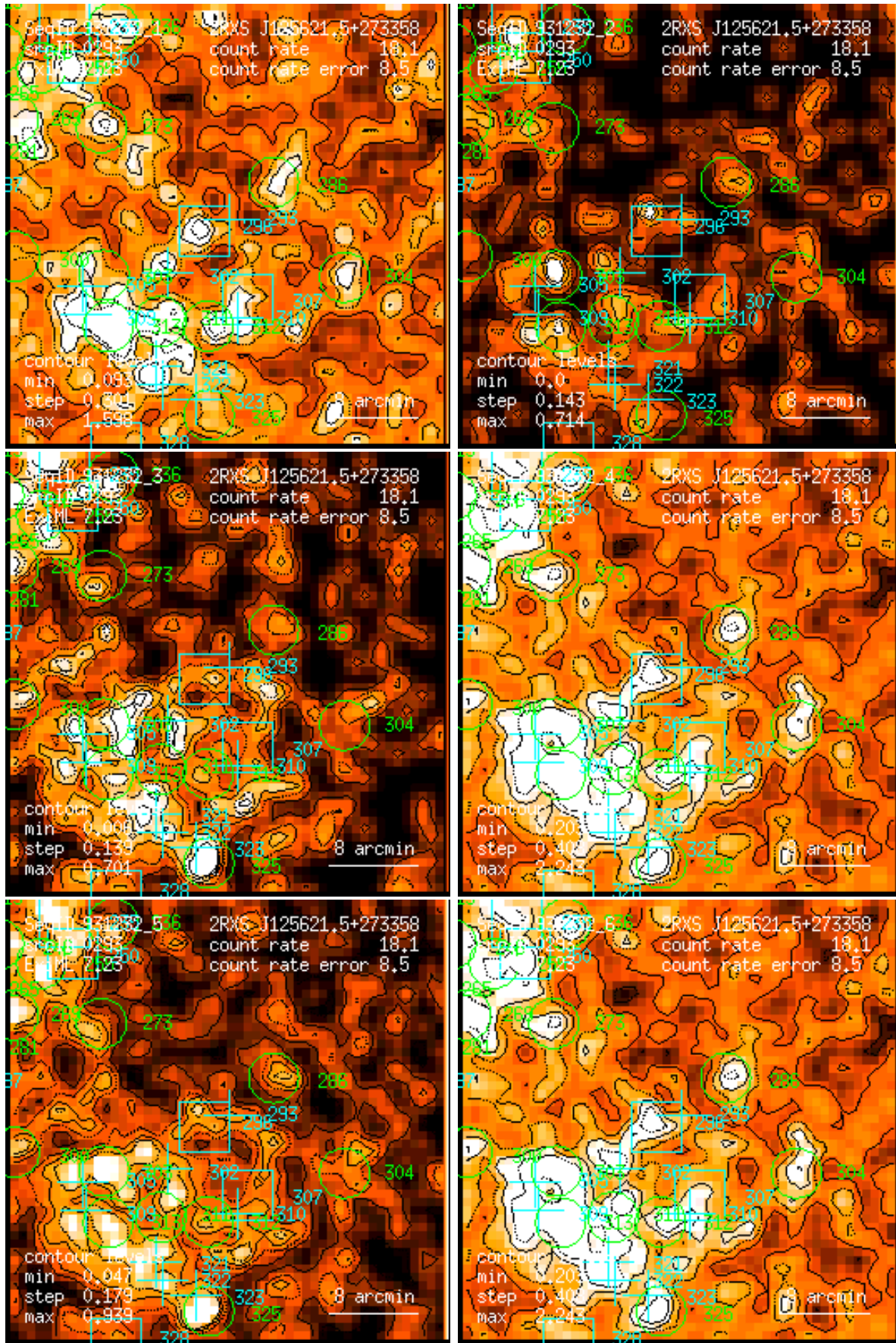
Figure 293: RASS 931232: detection 0293: band rate images, Gaussian filter: (1) PSPC channels 11 – 41, (2) 52 – 90, (3) 91 – 201, (4) 11 – 235, (5) 52 – 201, (6) 11 – 201. Broad band rates in counts/ks. Band rate contour levels in counts/ks/arcmin 2 .
