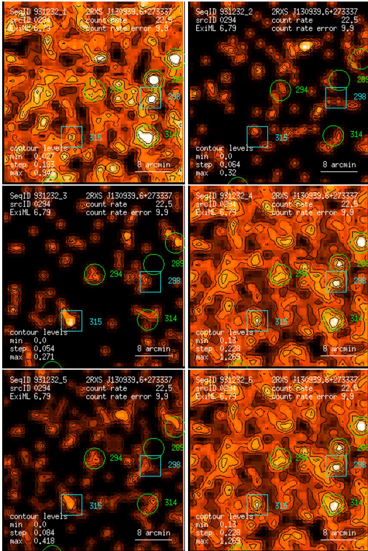
Figure 294: RASS 931232: detection 0294: band rate images, Gaussian filter: (1) PSPC channels 11 – 41, (2) 52 – 90, (3) 91 – 201, (4) 11 – 235, (5) 52 – 201, (6) 11 – 201. Broad band rates in counts/ks. Band rate contour levels in counts/ks/arcmin 2 .
