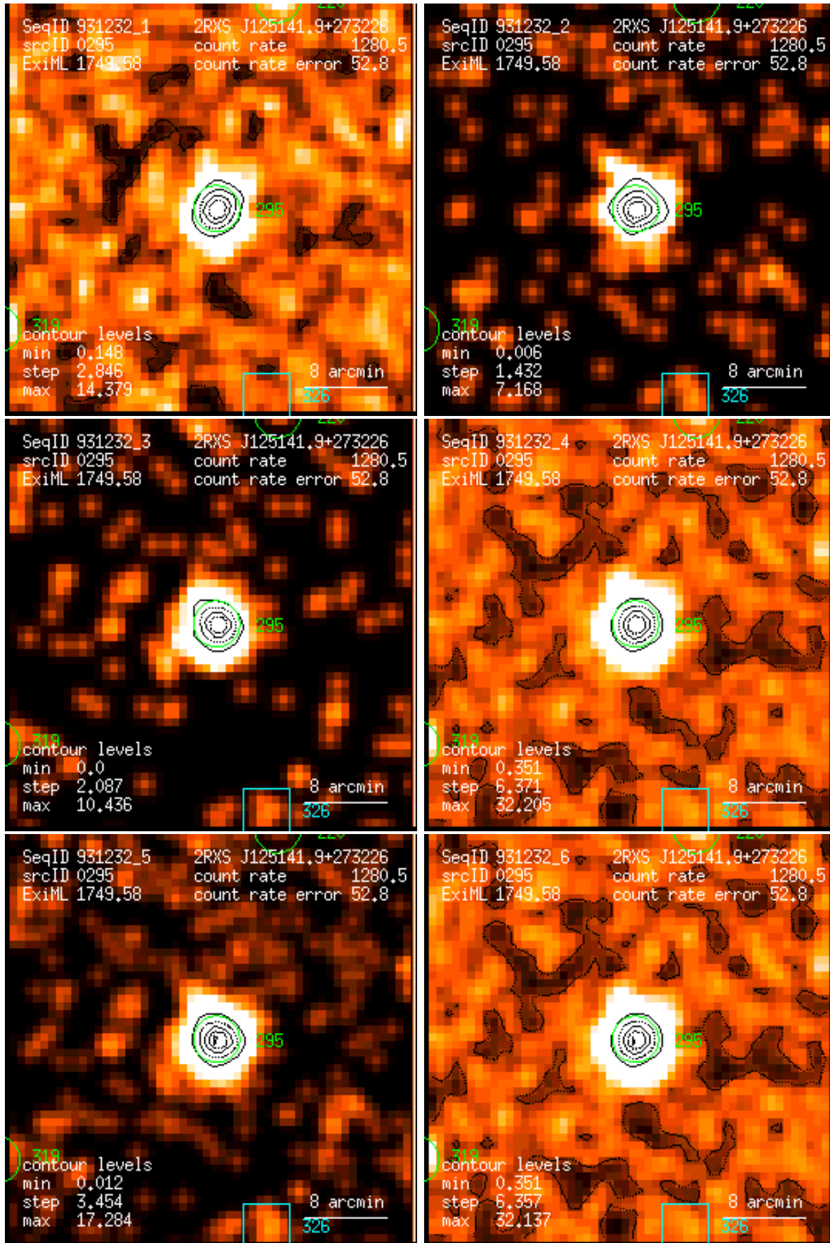
Figure 295: RASS 931232: detection 0295: band rate images, Gaussian filter: (1) PSPC channels 11 – 41, (2) 52 – 90, (3) 91 – 201, (4) 11 – 235, (5) 52 – 201, (6) 11 – 201. Broad band rates in counts/ks. Band rate contour levels in counts/ks/arcmin 2 .
