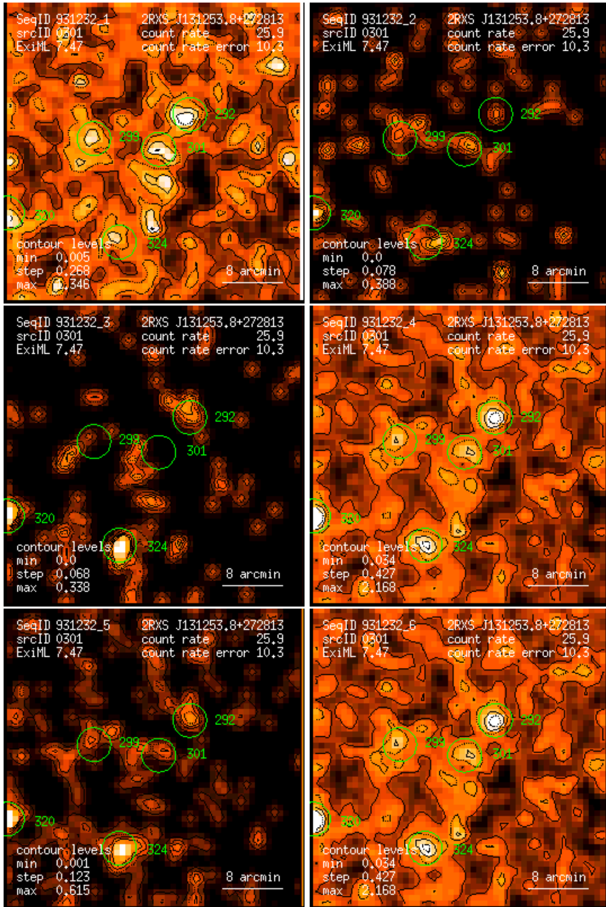
Figure 301: RASS 931232: detection 0301: band rate images, Gaussian filter: (1) PSPC channels 11 – 41, (2) 52 – 90, (3) 91 – 201, (4) 11 – 235, (5) 52 – 201, (6) 11 – 201. Broad band rates in counts/ks. Band rate contour levels in counts/ks/arcmin 2 .
