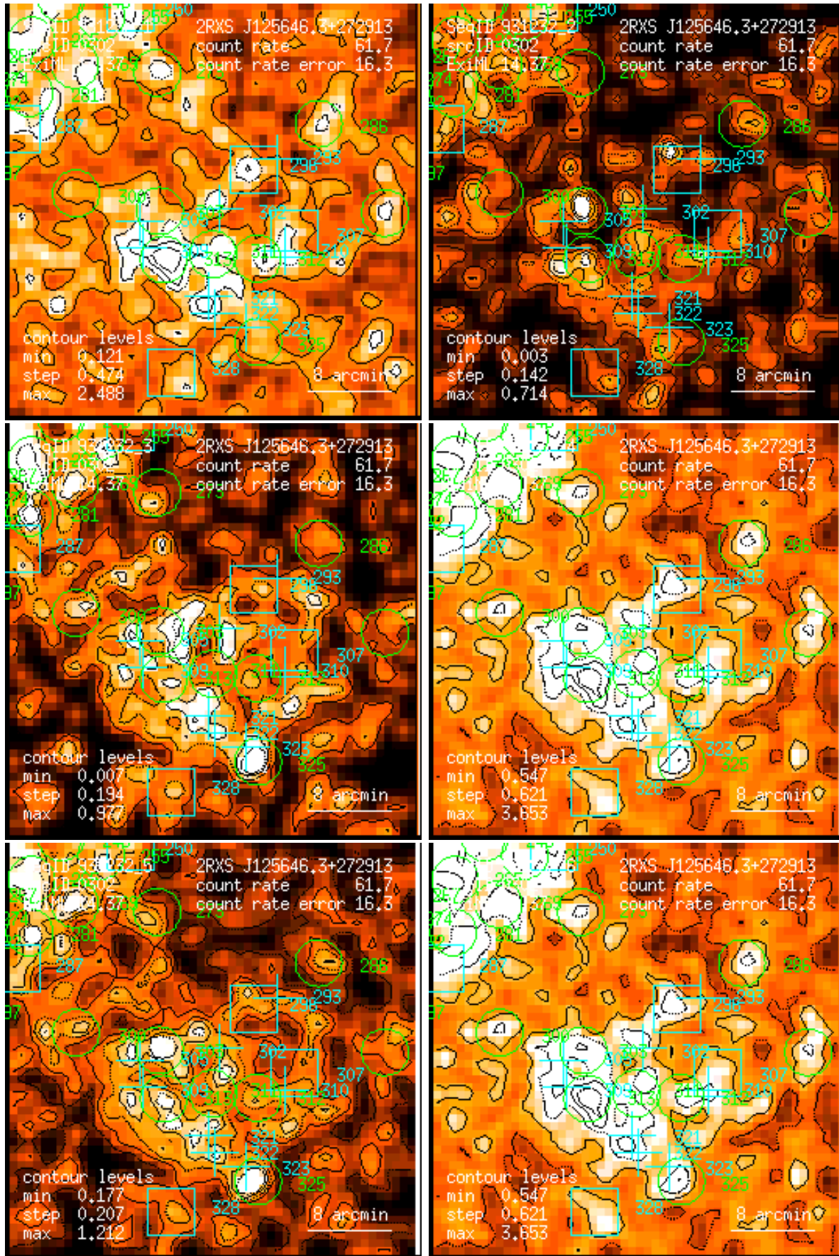
Figure 302: RASS 931232: detection 0302: band rate images, Gaussian filter: (1) PSPC channels 11 – 41, (2) 52 – 90, (3) 91 – 201, (4) 11 – 235, (5) 52 – 201, (6) 11 – 201. Broad band rates in counts/ks. Band rate contour levels in counts/ks/arcmin 2 .
