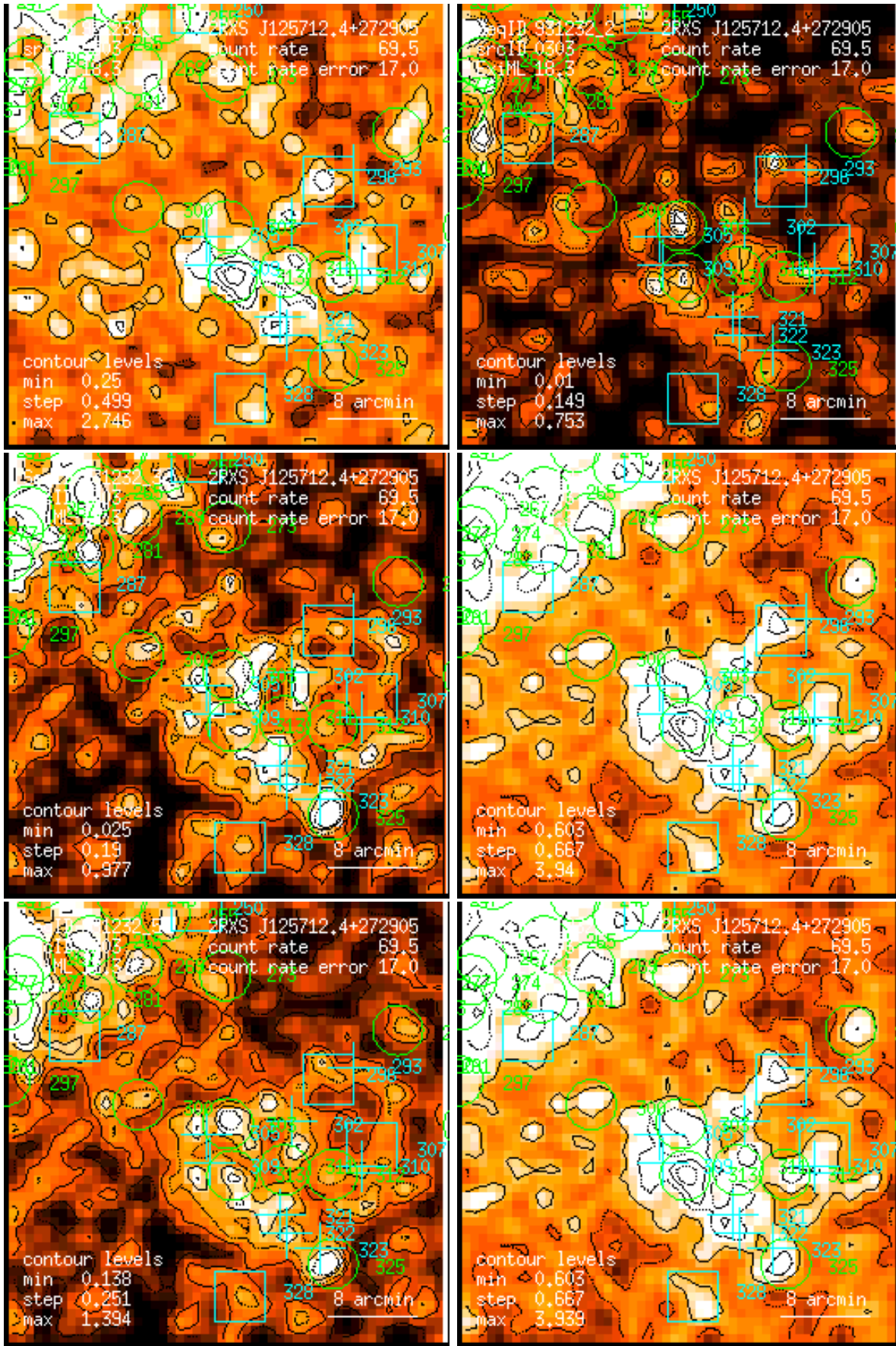
Figure 303: RASS 931232: detection 0303: band rate images, Gaussian filter: (1) PSPC channels 11 – 41, (2) 52 – 90, (3) 91 – 201, (4) 11 – 235, (5) 52 – 201, (6) 11 – 201. Broad band rates in counts/ks. Band rate contour levels in counts/ks/arcmin 2 .
