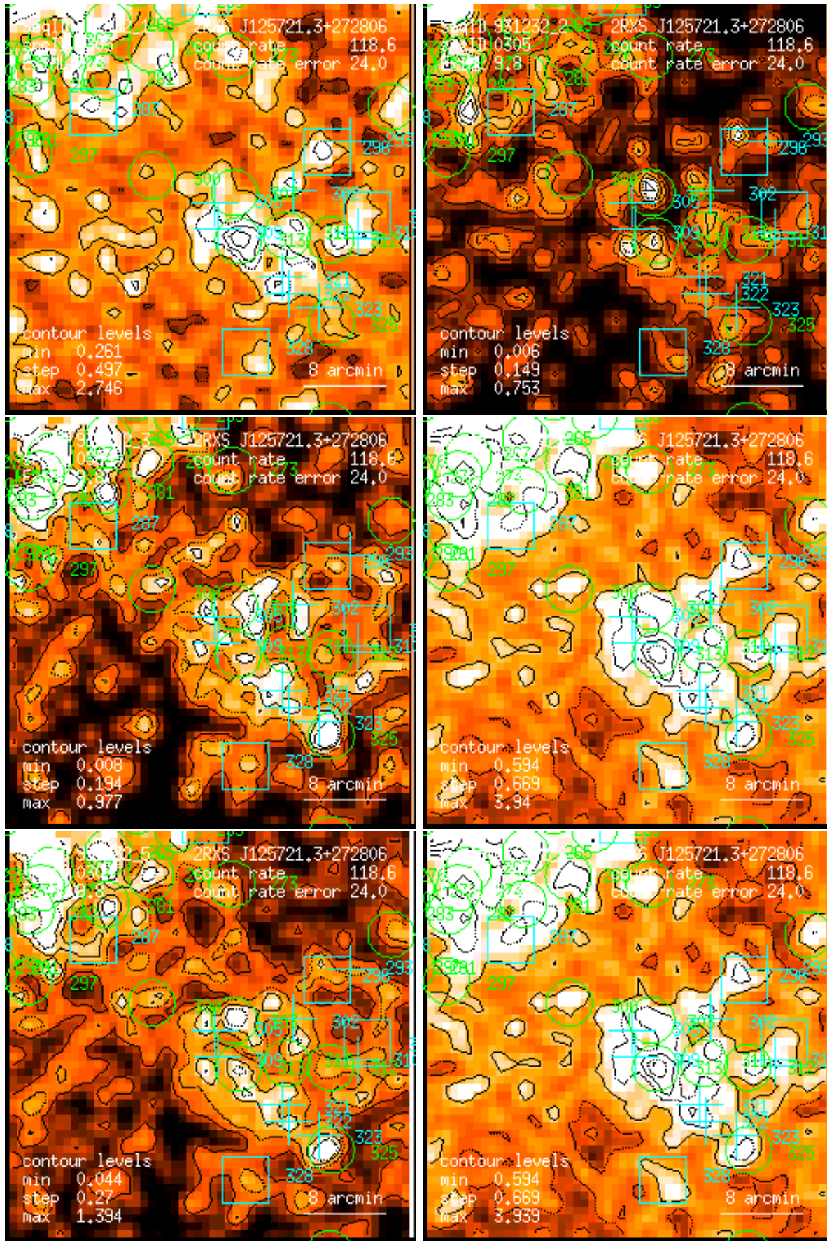
Figure 305: RASS 931232: detection 0305: band rate images, Gaussian filter: (1) PSPC channels 11 – 41, (2) 52 – 90, (3) 91 – 201, (4) 11 – 235, (5) 52 – 201, (6) 11 – 201. Broad band rates in counts/ks. Band rate contour levels in counts/ks/arcmin 2 .
